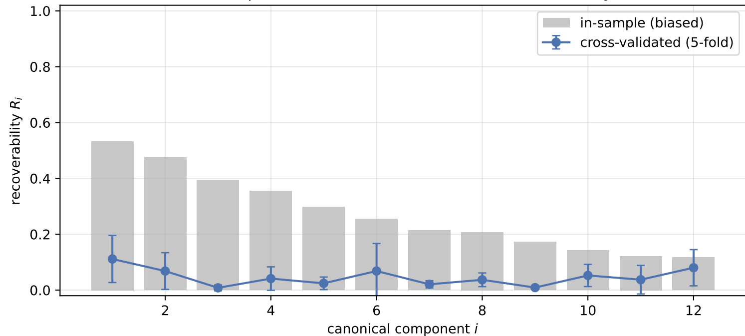
In-sample vs. honest (cross-validated) recoverability
