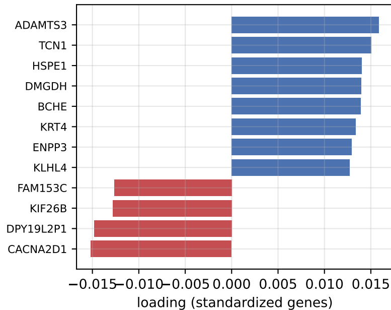
direction a_2 ( R_2 = 0.48 )
