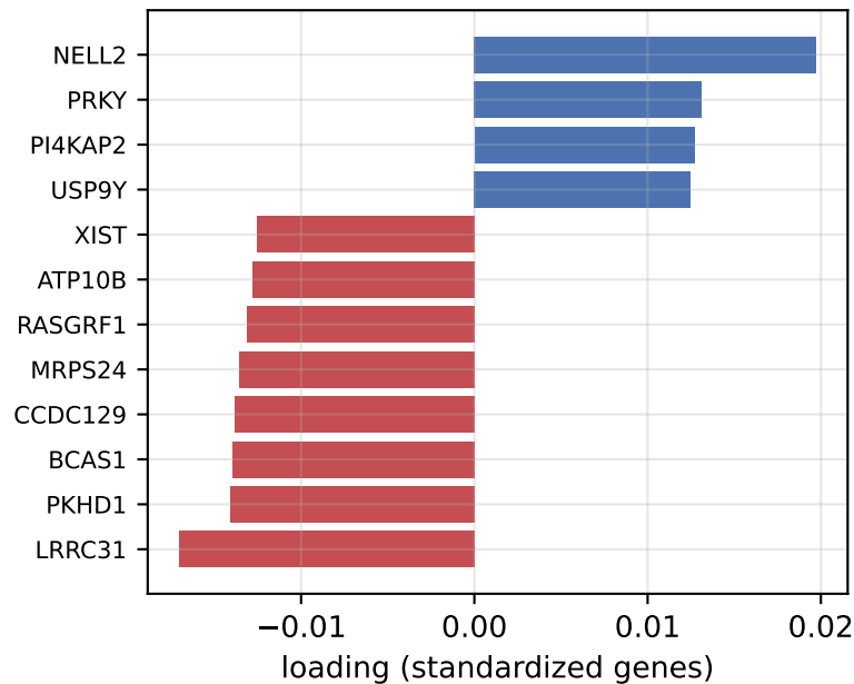
direction a_1 ( R_1 = 0.53 )
