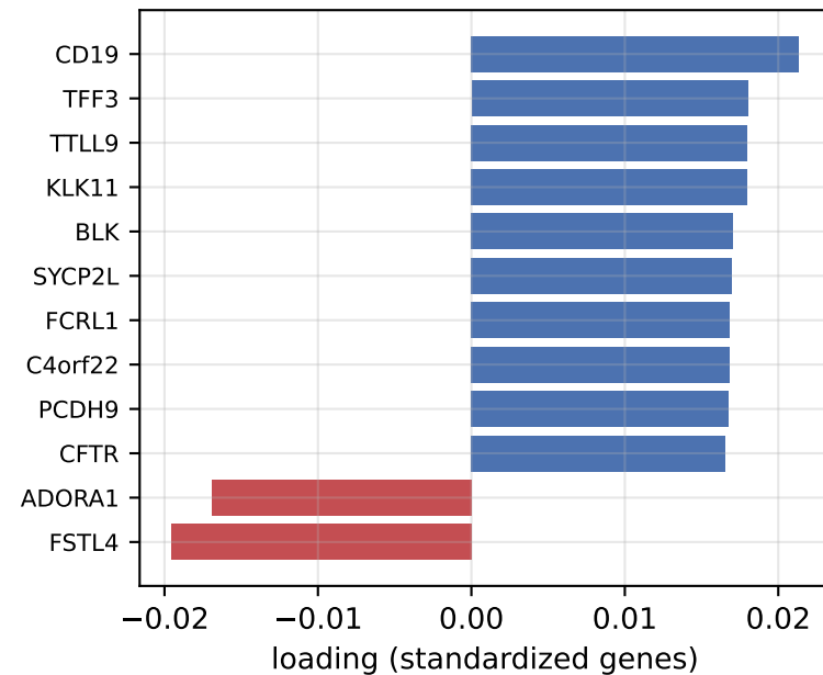
direction a_3 ( R_3 = 0.39 )
