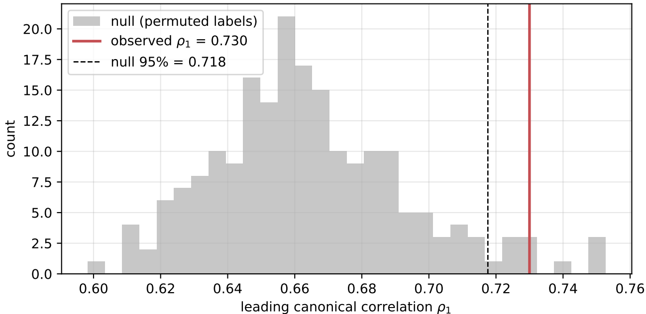
Permutation null (n = 200)
