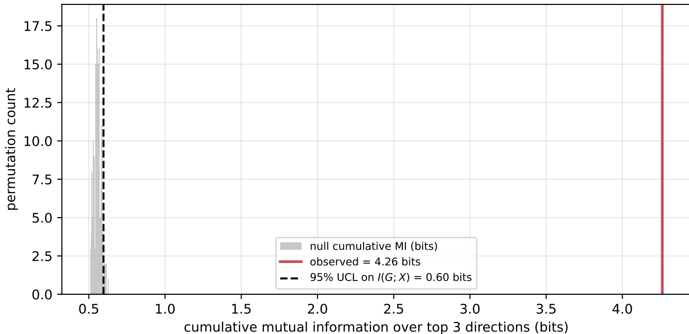
Upper-bound on I(G; X) from the permutation null
