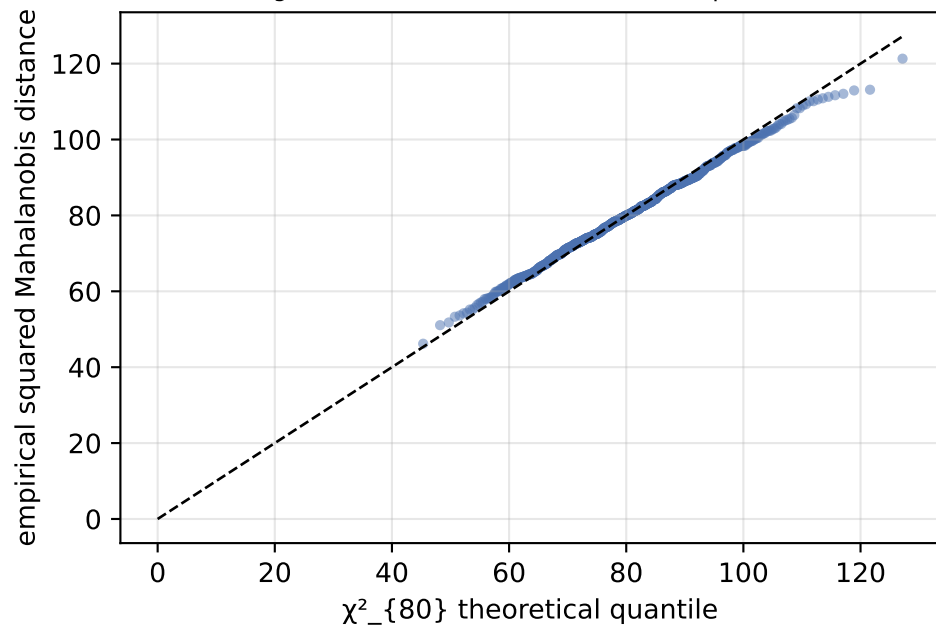
genomics — raw features (n=800 > p=80)
