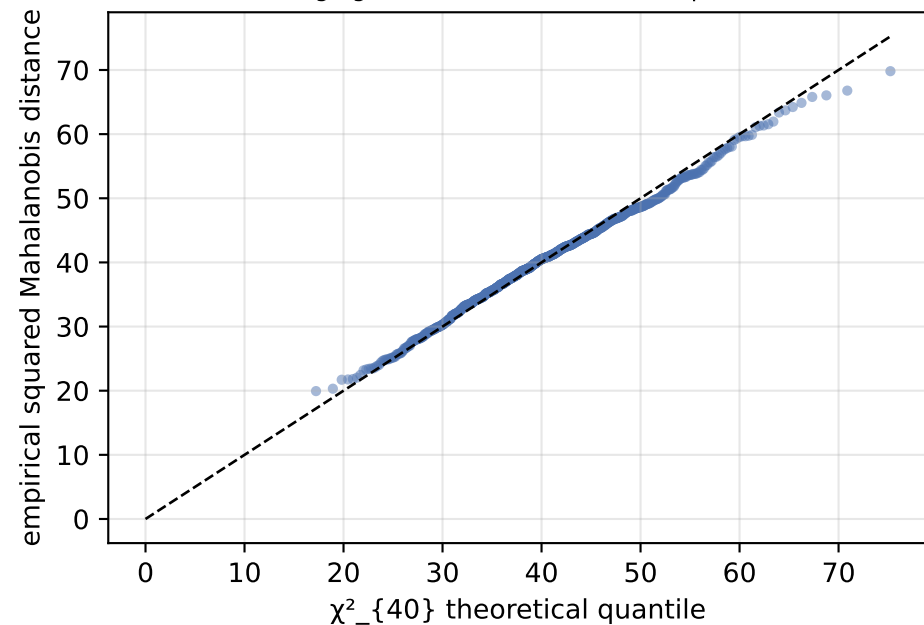
imaging — raw features (n=800 > p=40)
