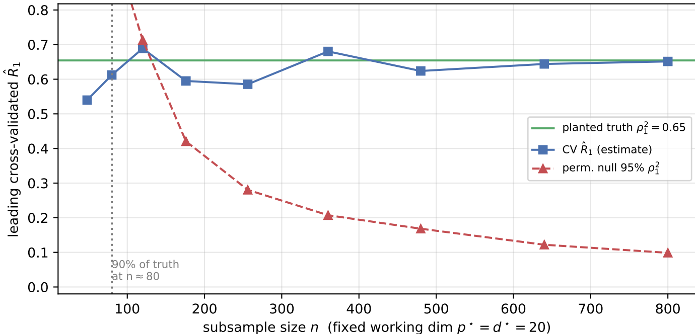
Synthetic data: CV recoverability vs. subsample size, known truth
