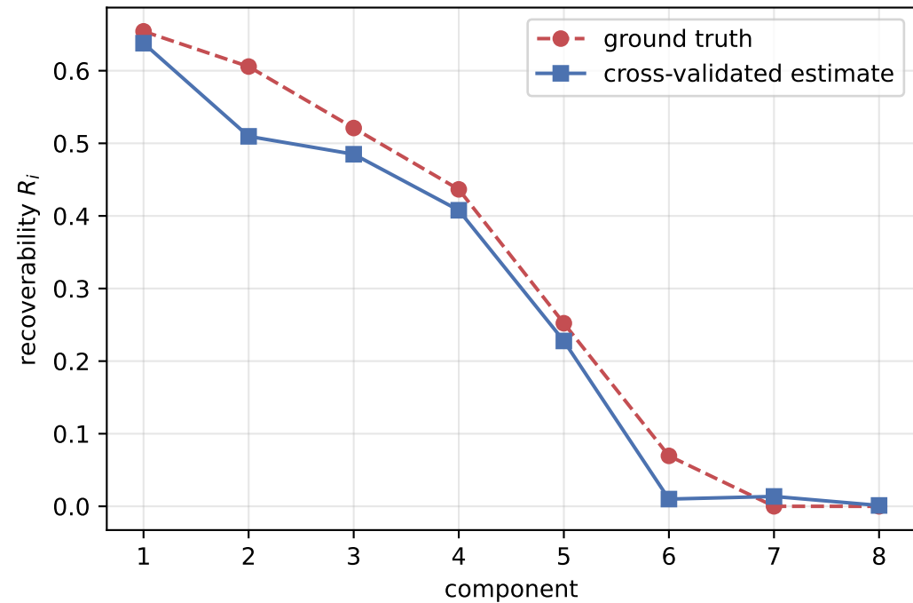
Estimated vs. true recoverability
