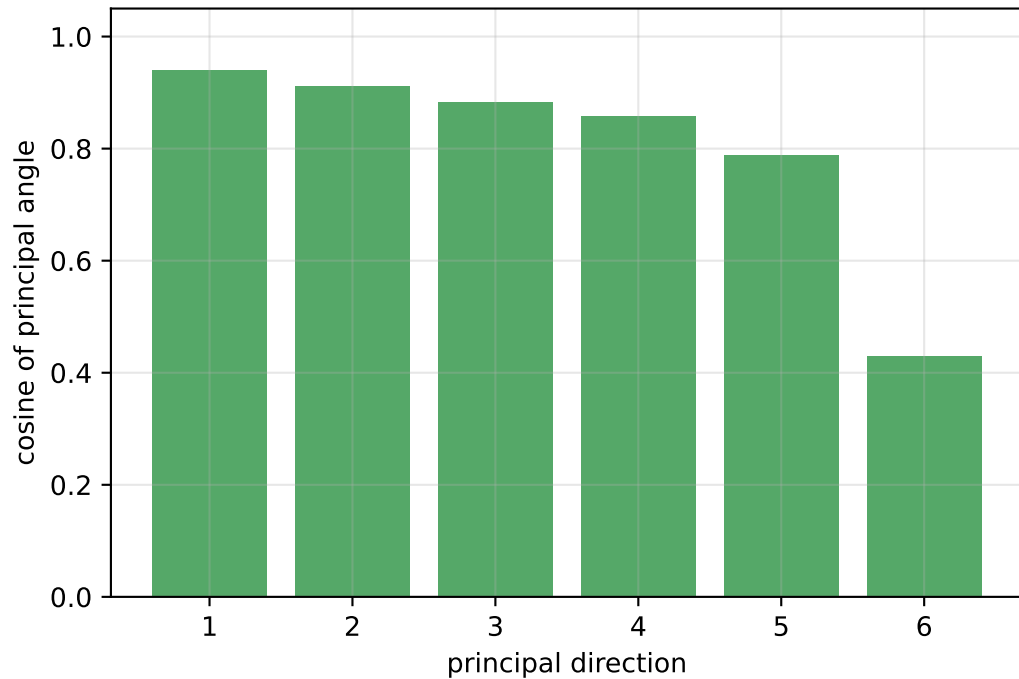
Estimated vs. true genomic subspace
