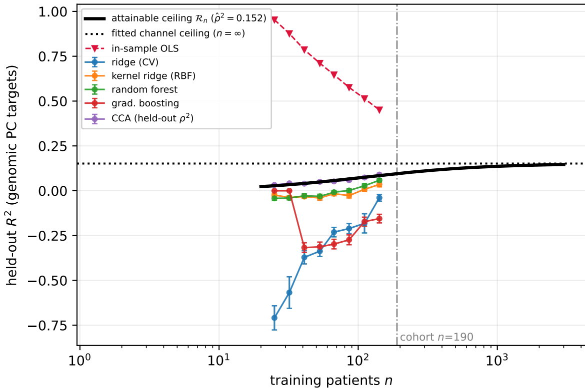
KIRC: trained models vs. the attainable ceiling
