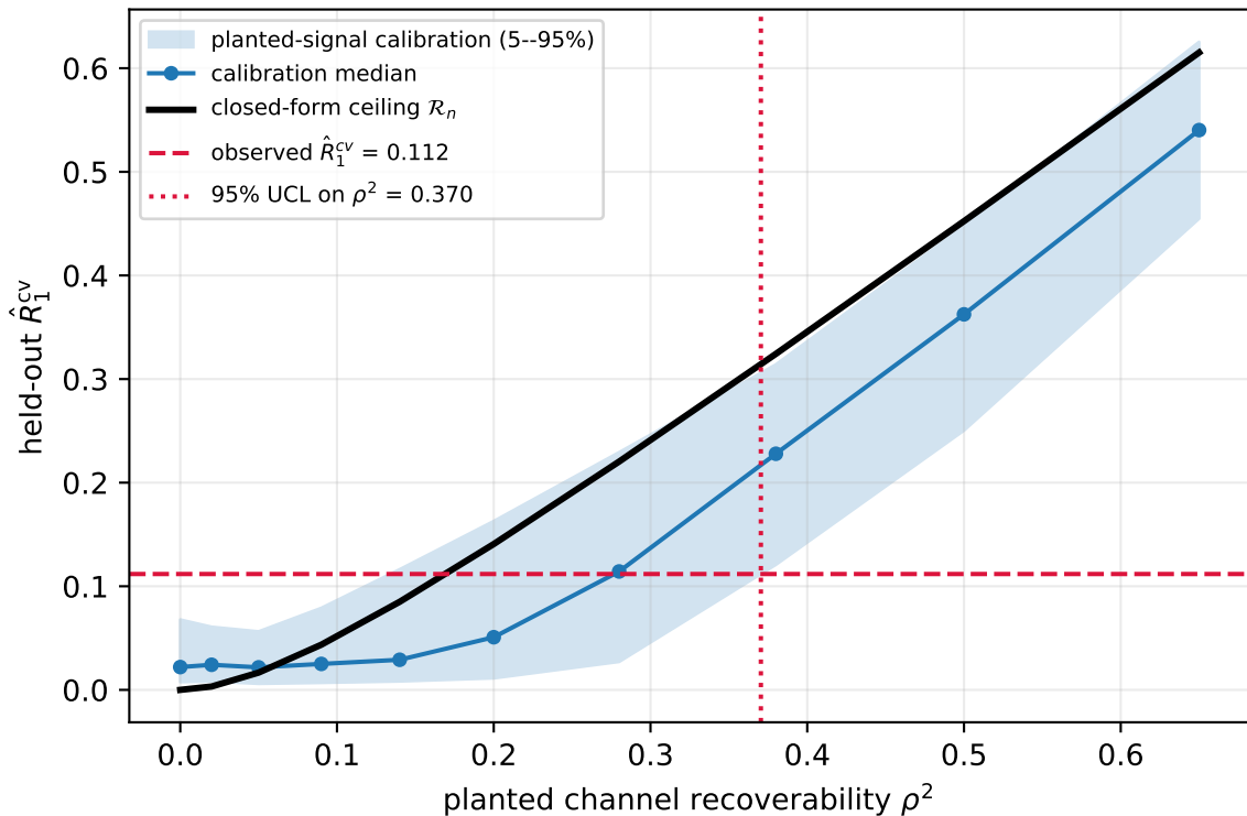
KIRC: channel UCL by test inversion (n=190)
