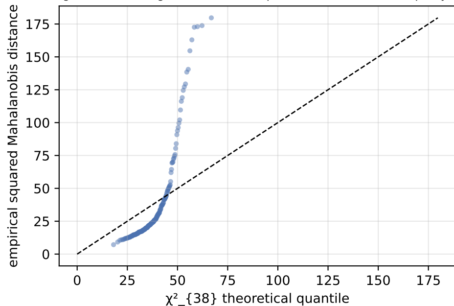
genomics — 38 genomic PCs (raw p=2000 \geq n=190, PCA proxy)
