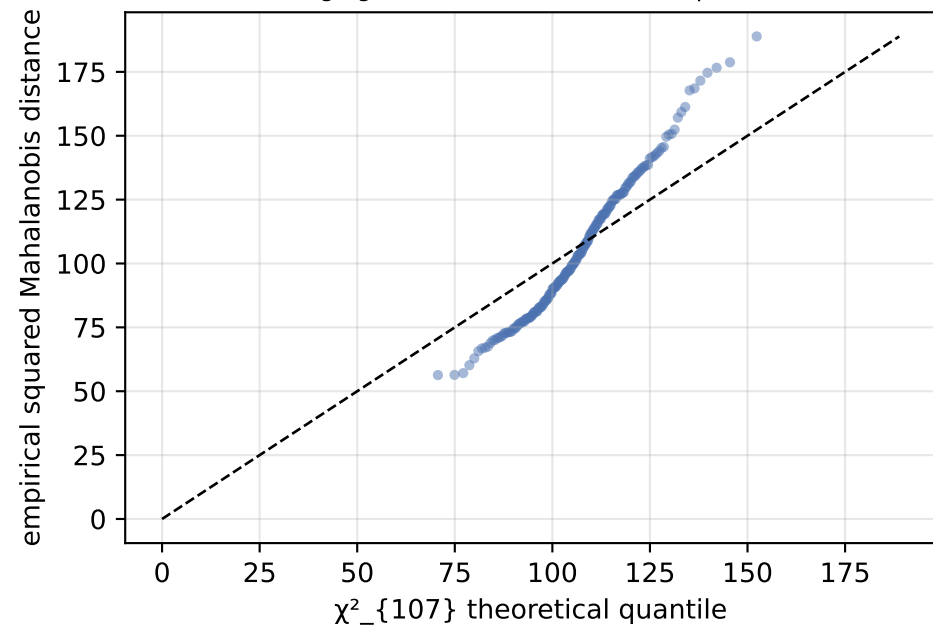
imaging — raw features (n=190 > p=107)
