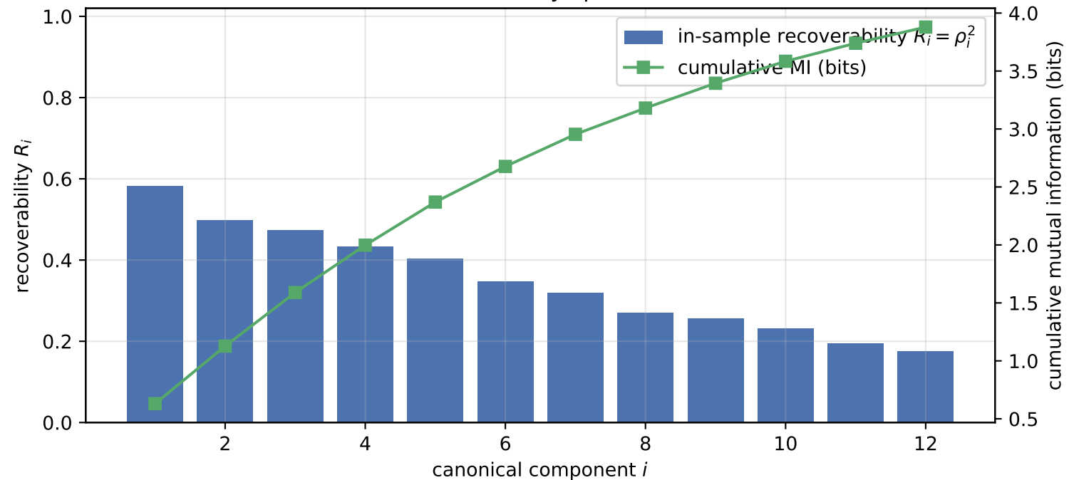
Recoverability spectrum
