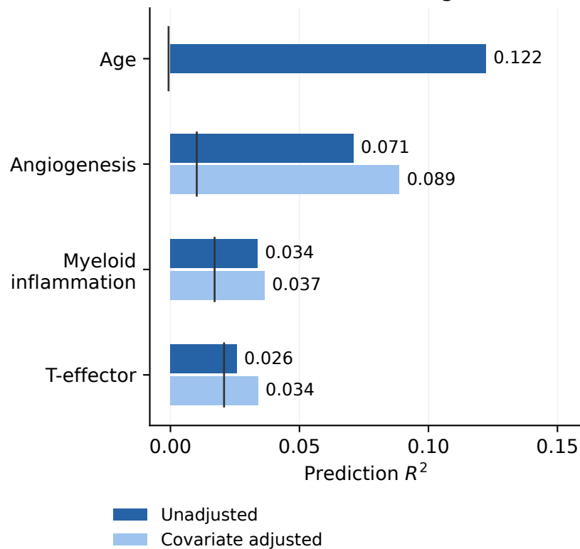
b Continuous targets
