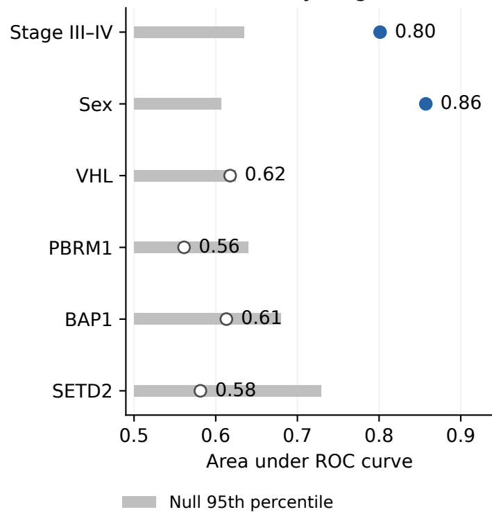
a Binary targets
