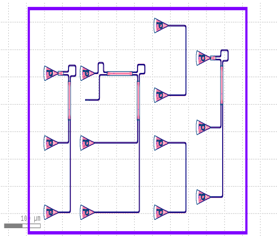
Fig. 9: PIC Layout
