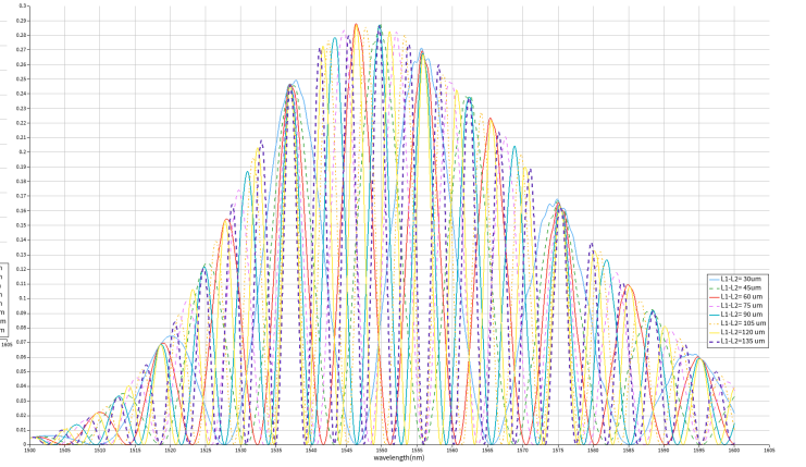
Fig. 8. Transmission spectra of unbalanced MZIs with different \Delta L ( 500 \text{ nm} \times 220 \text{ nm} strip waveguide, TE).
