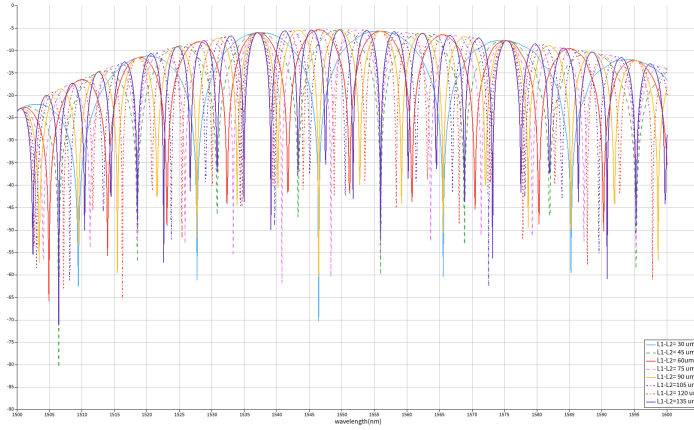
Fig. 6. Optical spectra of unbalanced MZIs with different \Delta L ( 500 \text{ nm} \times 220 \text{ nm} strip waveguide, TE).
