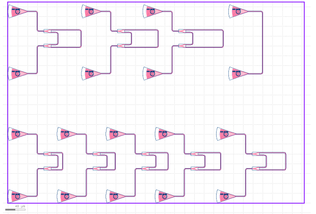
Fig. 9. Layout of the [605 \times 410] \mu\text{m} cell showing the unbalanced MZIs, calibrator and their grating couplers.
