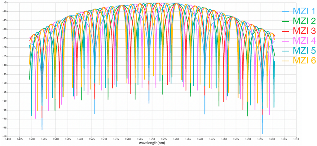
Figure 3: Simulated Transmission Spectrum (dB) vs. Wavelength for MZI Variations ( \Delta L = 25 \mu m to 150 \mu m ) showing interference fringes and grating coupler envelope.
