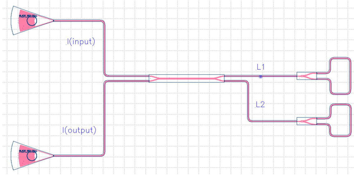
Fig. 11. Michelson Interferometer structure
