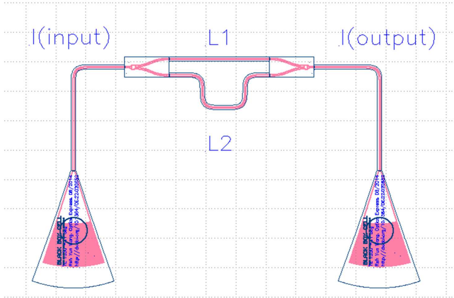
Fig. 8. MZI structure
