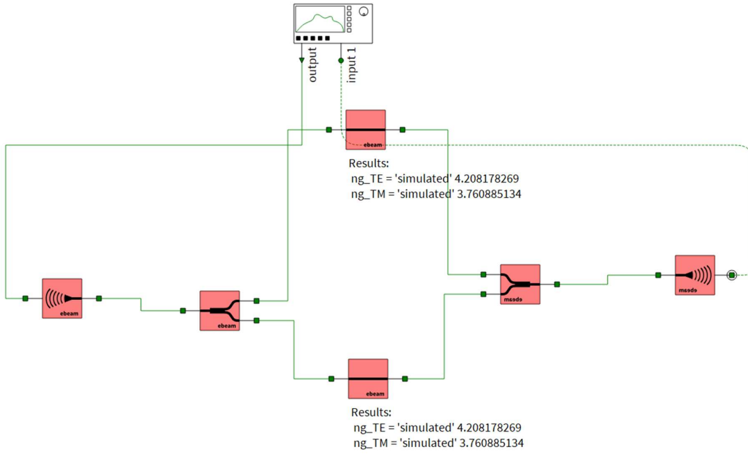
Fig. 10. Simulation of MZI structure with Grating Coupler
