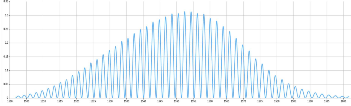
Fig. 9. Transmission Spectrum of MZI structure with Grating Coupler
