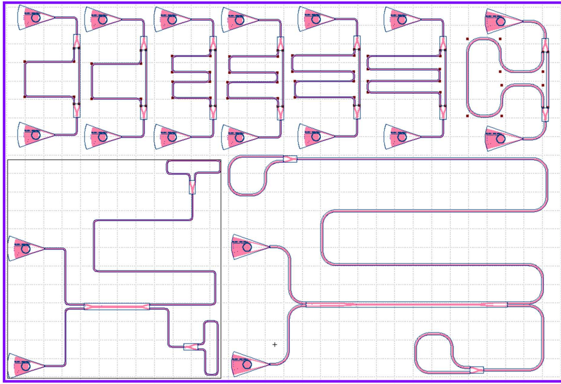
Fig. 13. Layout of the complete photonic test structures.
