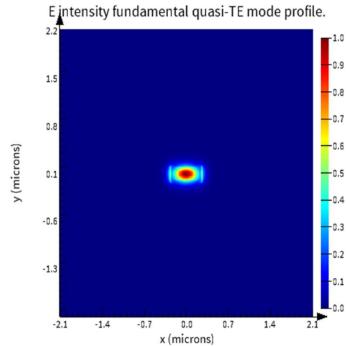
Fig. 3. Simulated fundamental quasi-TE mode profile.
