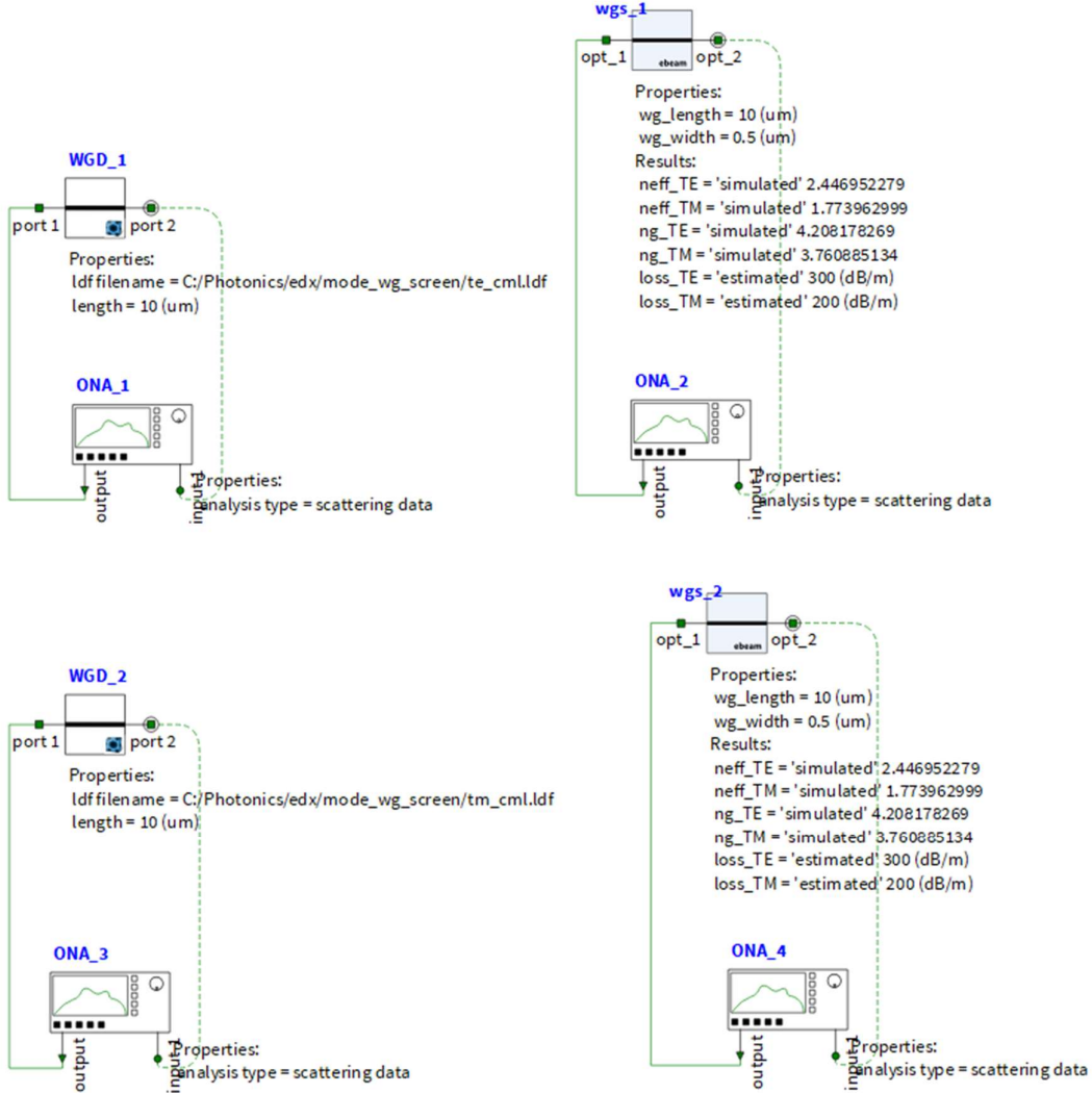
Fig. 7. Lumerical IC setup for CML validation
