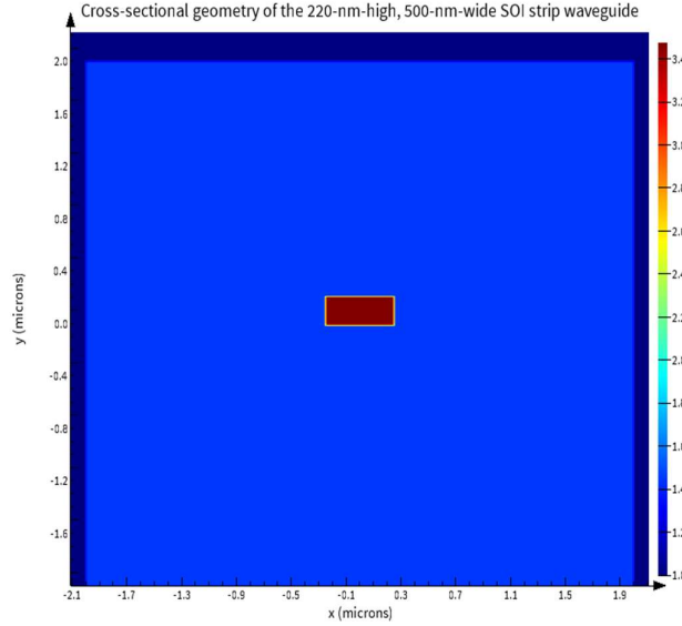
Fig. 1. Cross-sectional geometry of the 220-nm-high, 500-nm-wide SOI strip waveguide.
