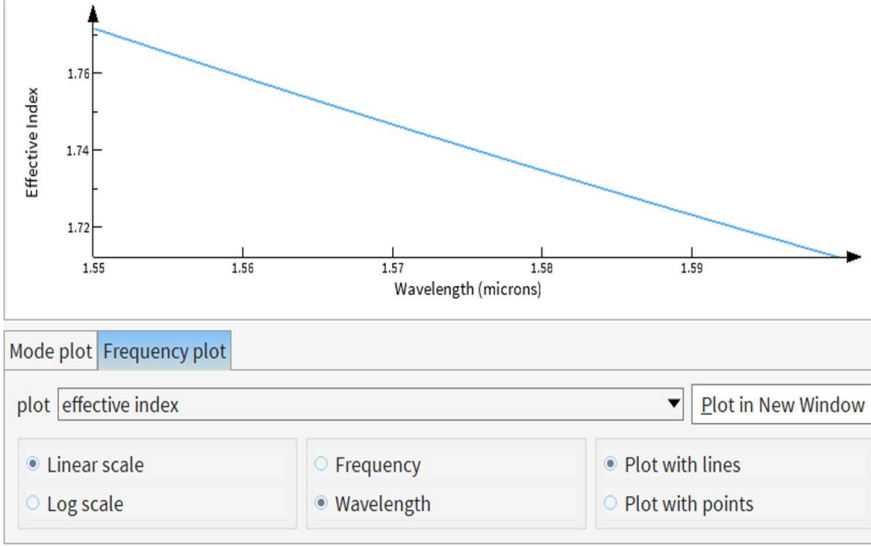
Fig. 6. Dispersion Analysis of fundamental quasi-TM mode.
