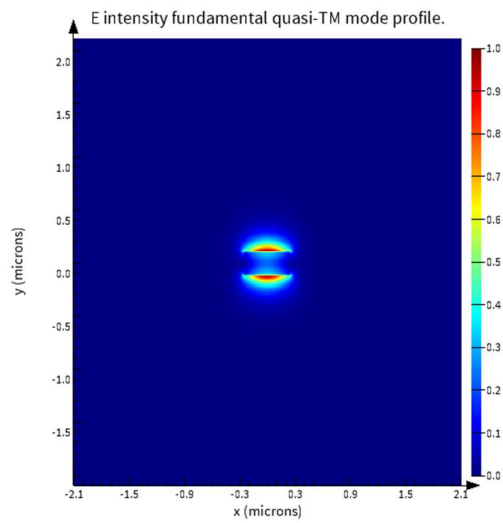
Fig. 4. Simulated fundamental quasi-TM mode profile.
