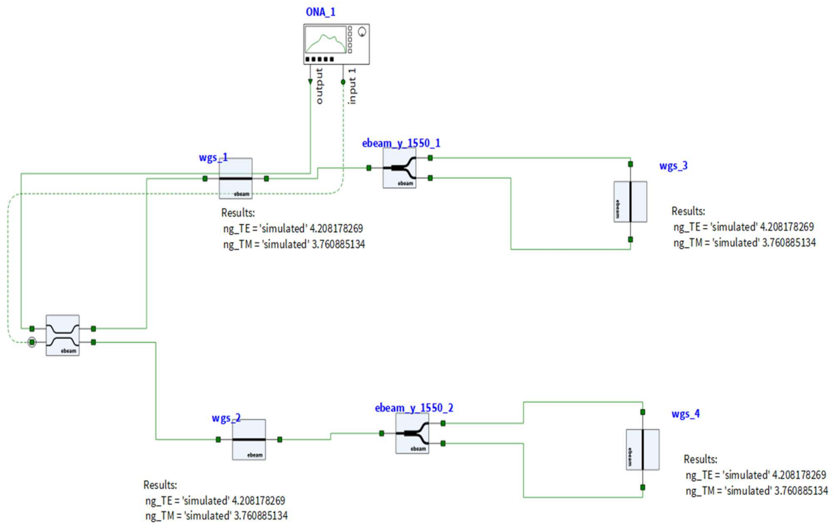
Fig. 12. Simulation of Michelson Interferometer structure
