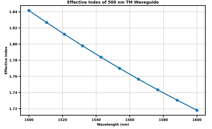
Fig. 7. n_{\text{eff}} of a 500 nm x 220 nm crosssection of a Si waveguide in SiO 2 cladding of the quasi-TM mode 1.
