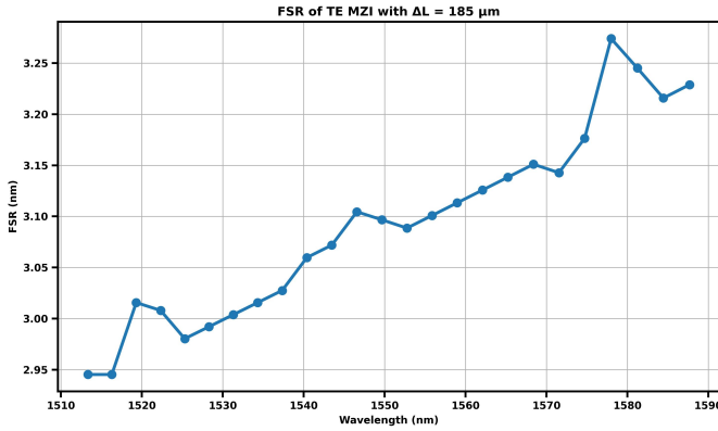
Fig. 11. FSR of MZI3 (TE, \Delta L = 185\mu m ).
