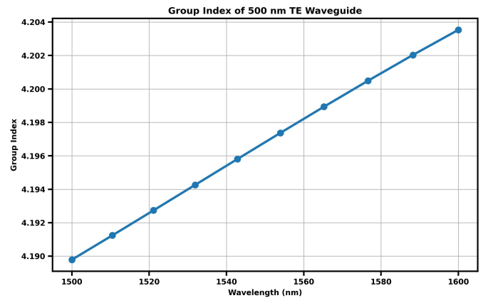
Fig. 4. n_g of a 500 nm x 220 nm crosssection of a Si waveguide in SiO 2 cladding of the quasi-TE mode 1.
