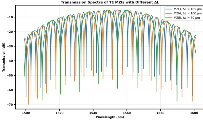
Fig. 10. Spectra of 3 standard TE MZIs with different \Delta L .
