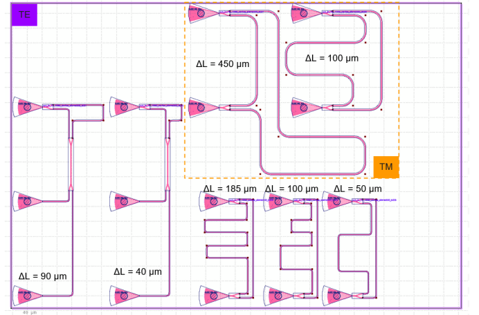
Fig. 9. Floor plan with various MZI devices. Every device in the purple box is TE except for those enclosed in the orange dashed box, which is TM.
