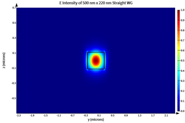
Fig. 1. E intensity of a 500 nm x 220 nm crosssection of a Si waveguide in SiO 2 cladding of the quasi-TE mode 1.
