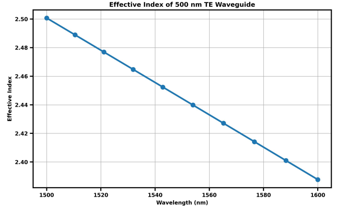
Fig. 3. n_{eff} vs wavelength of a 500 nm x 220 nm crosssection of a Si waveguide in SiO 2 cladding of the quasi-TE mode 1.
