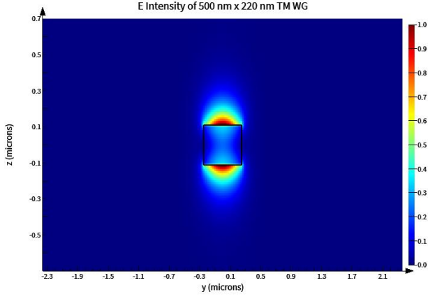
Fig. 5. E intensity of a 500 nm x 220 nm crosssection of a Si waveguide in SiO 2 cladding of the quasi-TM mode 1.
