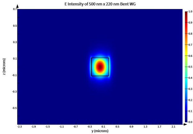
Fig. 2. E intensity of a 500 nm x 220 nm crosssection of a bent Si waveguide in SiO 2 cladding of the quasi-TE mode 1.
