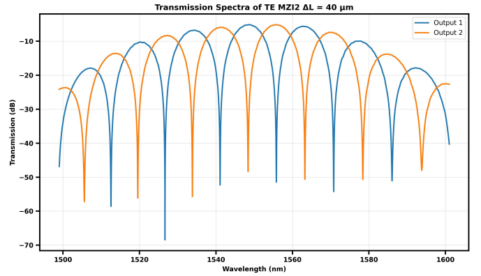
Fig. 13. Spectra of MZI2 (TE, \Delta L = 40\mu m ).
