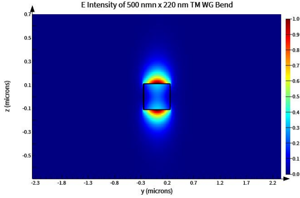
Fig. 6. E intensity of a 500 nm x 220 nm crosssection of a bent Si waveguide with bend radius 15 nm in SiO 2 cladding of the quasi-TM mode 1.
