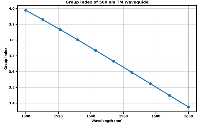
Fig. 8. n_g of a 500 nm x 220 nm crosssection of a Si waveguide in SiO 2 cladding of the quasi-TM mode 1.
