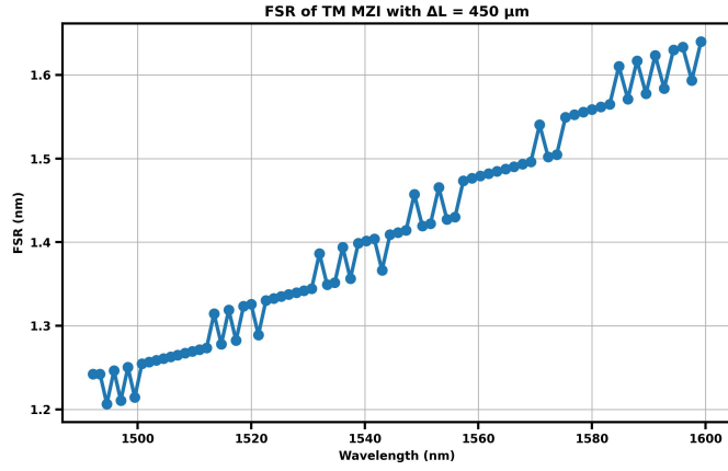
Fig. 16. FSR of MZI7 (TM, \Delta L = 450\mu m )
