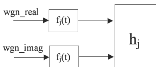
Figure E-2. Fading Tap Gain Generation
