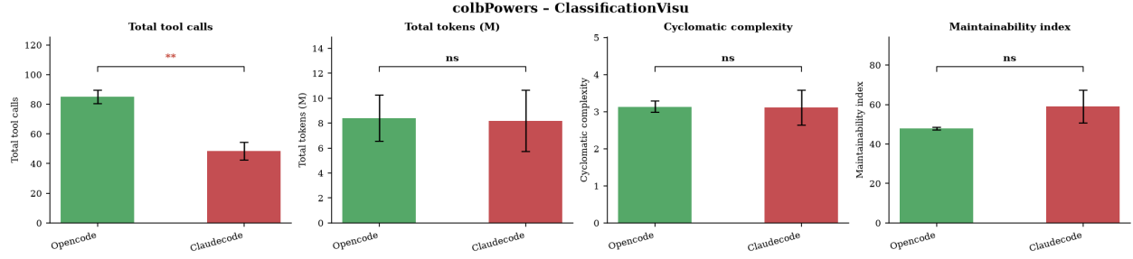
Figura 14: Test t de Welch — OpenCode vs. ClaudeCode, colbPowers, Caso 2.
