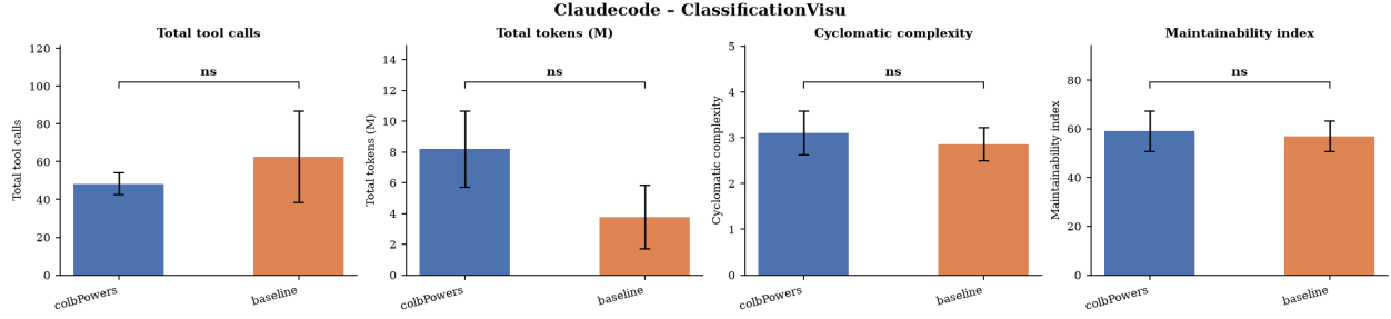
Figura 12: Test t de Welch — colbPowers vs. baseline, ClaudeCode, Caso 2.
