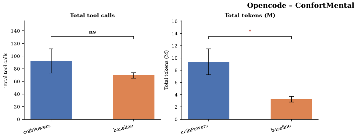
Figura 7: Test t de Welch — colbPowers vs. baseline, OpenCode, Caso 1.
