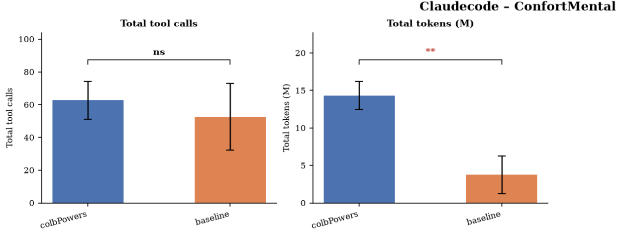
Figura 8: Test t de Welch — colbPowers vs. baseline, ClaudeCode, Caso 1.
