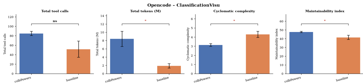
Figura 11: Test t de Welch — colbPowers vs. baseline, OpenCode, Caso 2 (* p < 0,05 ).
