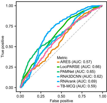
TM-score > 0.3 as success threshold
