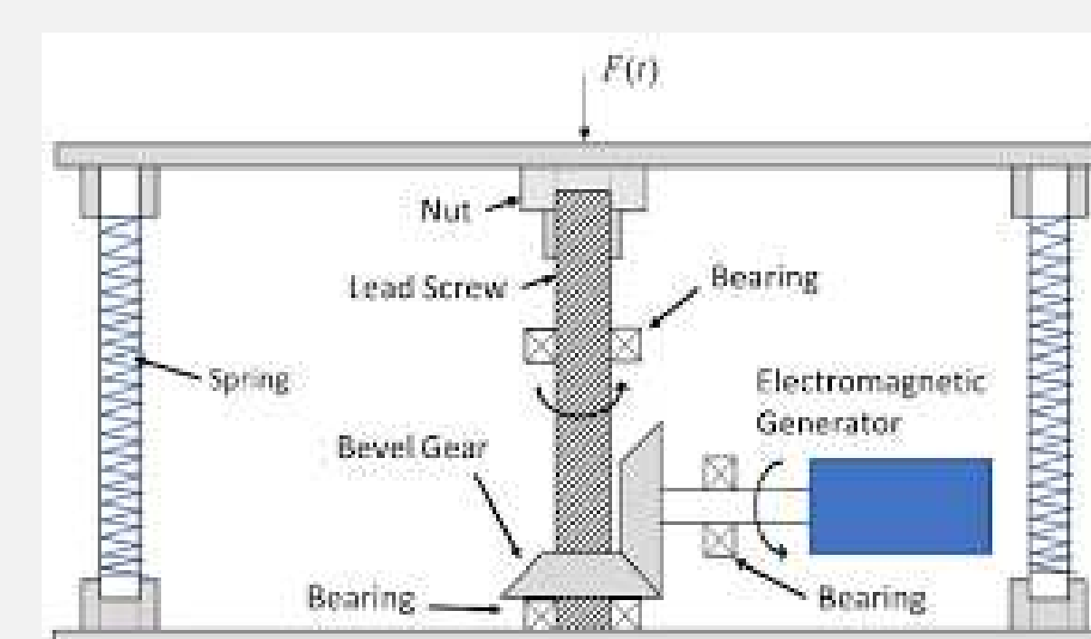
Screw Based Design with Electromagnetic Generator
