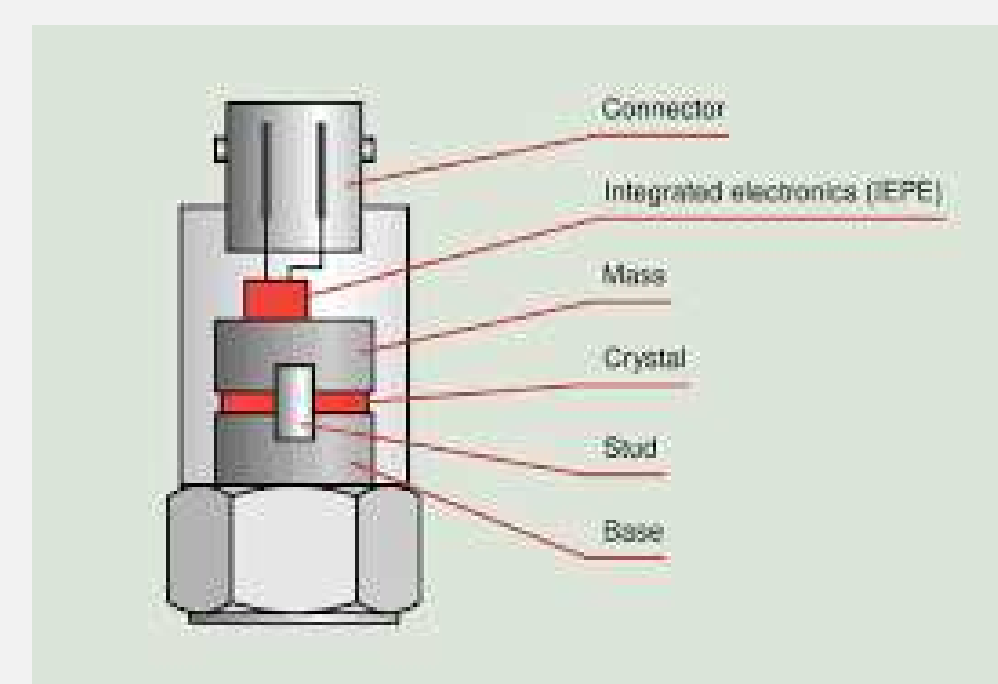
Piezoelectric Transducer
