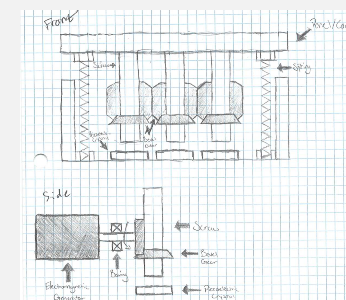
Prototype Design Sketch
