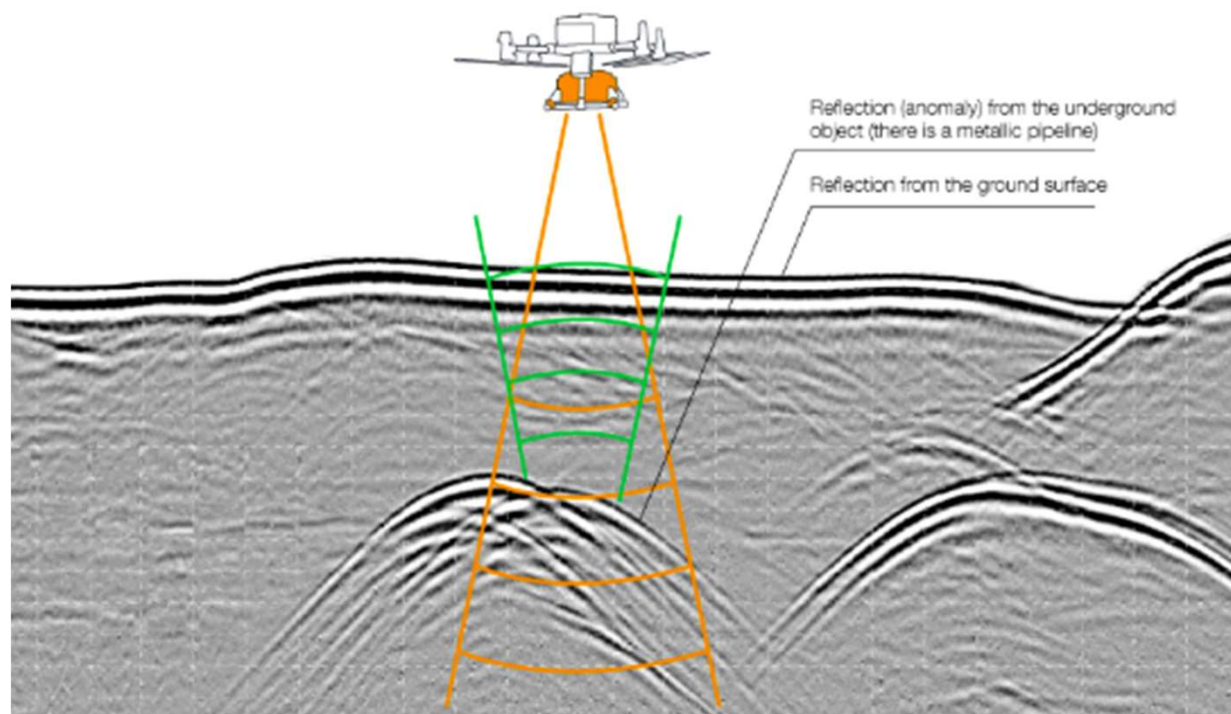
Drone- Mounted GPR Detecting underground Anomalies
