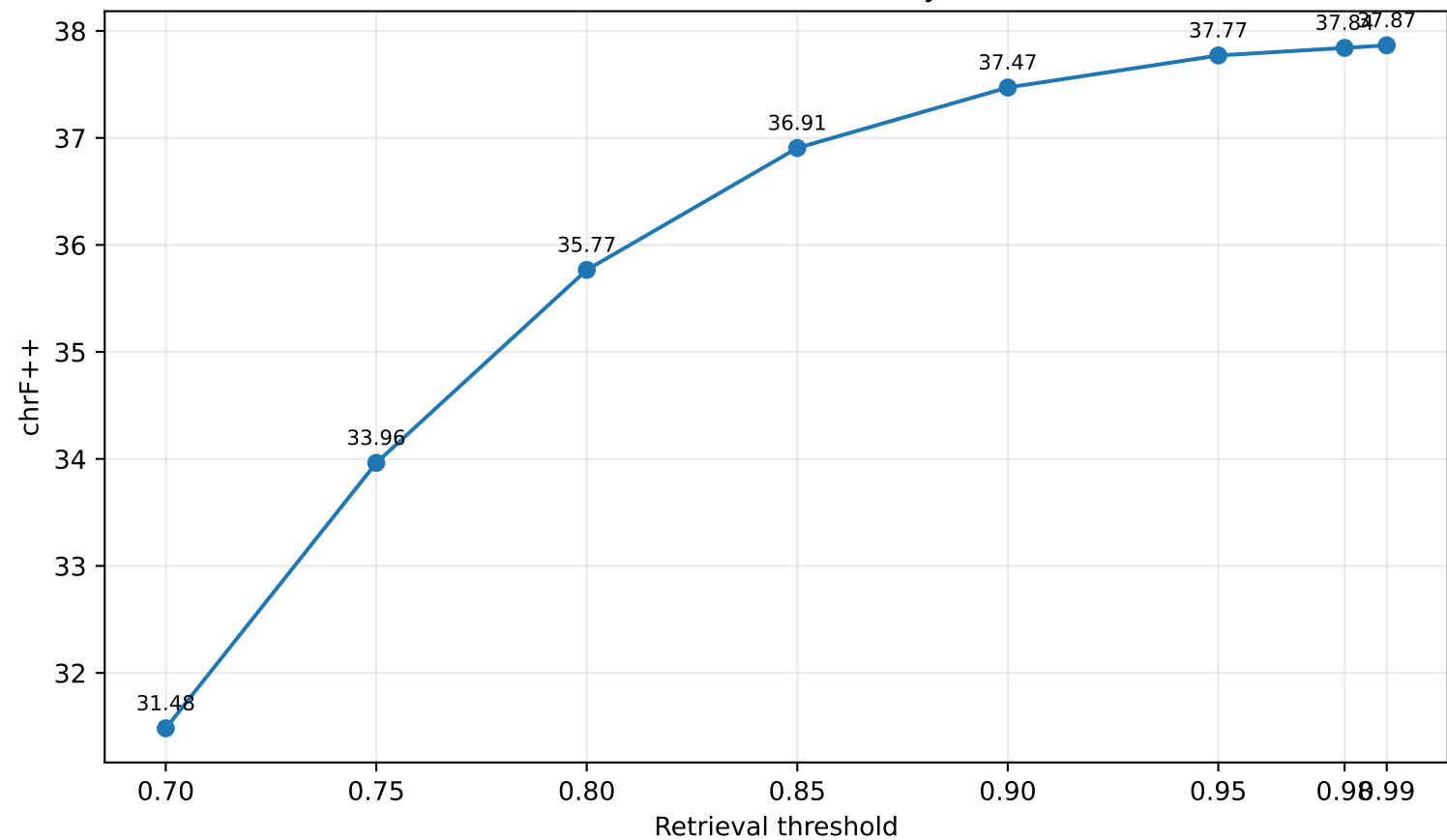
50K RAG Threshold Sensitivity: chrF++
