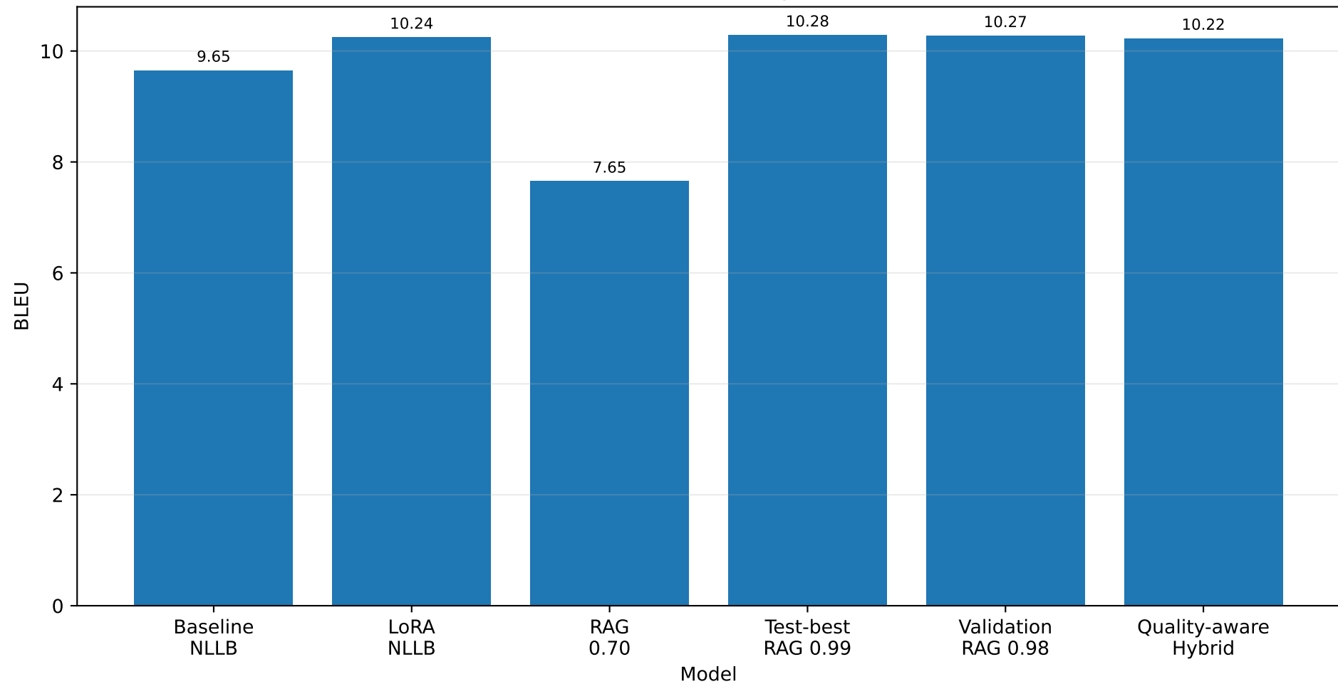
Final 50K BLEU Comparison
