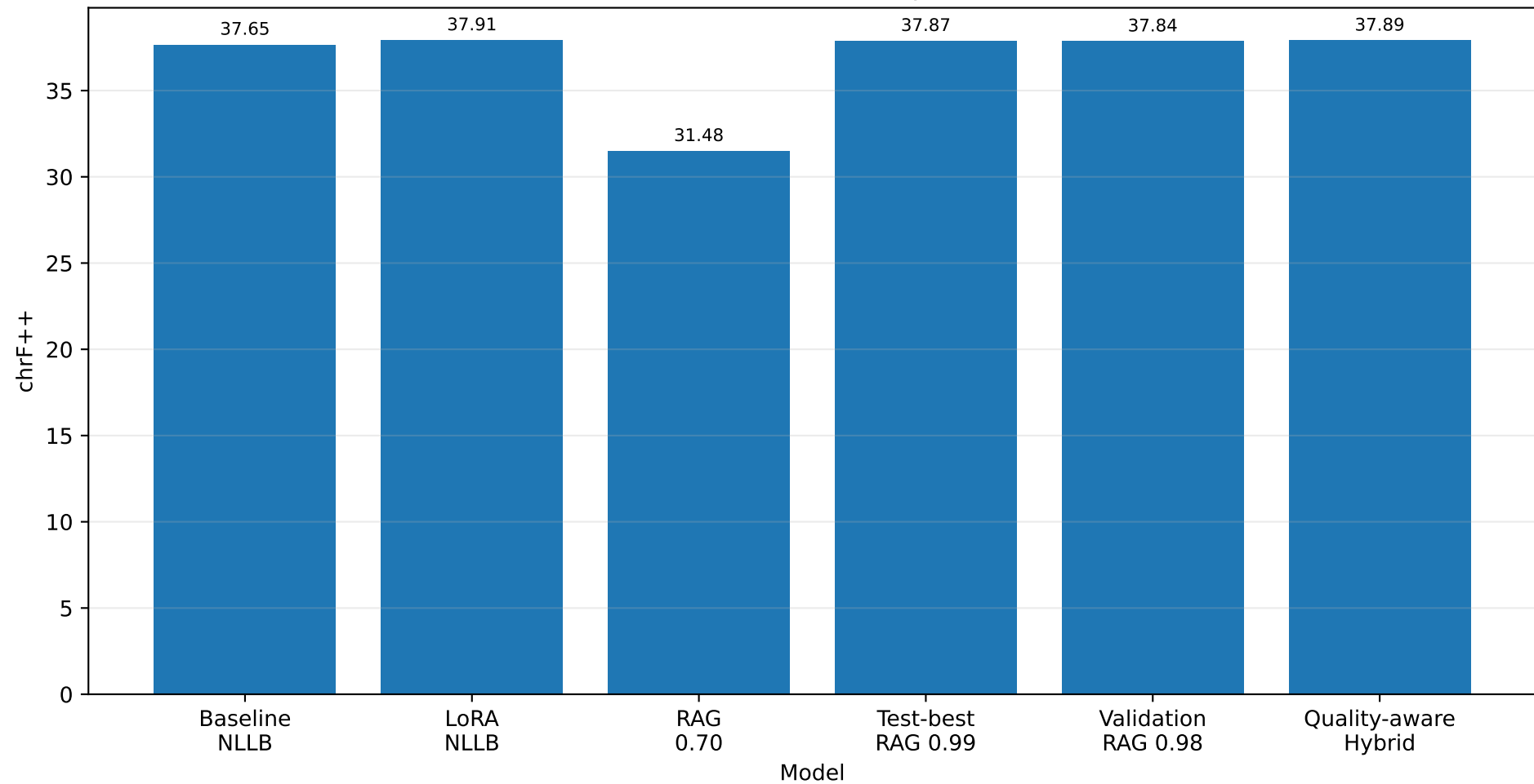
Final 50K chrF++ Comparison
