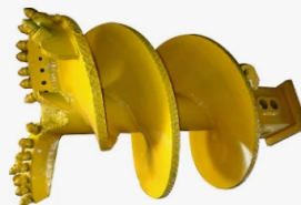
450mm Drilling Diameter Auger Drill Bit for Sale Can Customized
