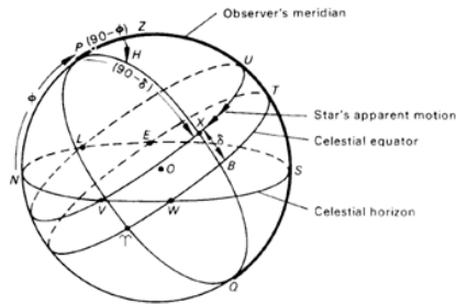
Gambar 2.3 Tata koordinat ekuatorial Sumber: Astronomy Principles and Practice
