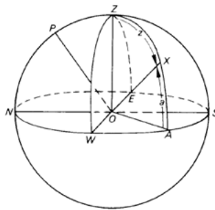
Gambar 2.2 Tata koordinat azimuth Sumber: Astronomy Principles and Practice
