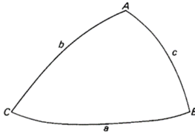
Gambar 2.1 Segitiga Bola Sumber: Astronomy Principles and Practice
