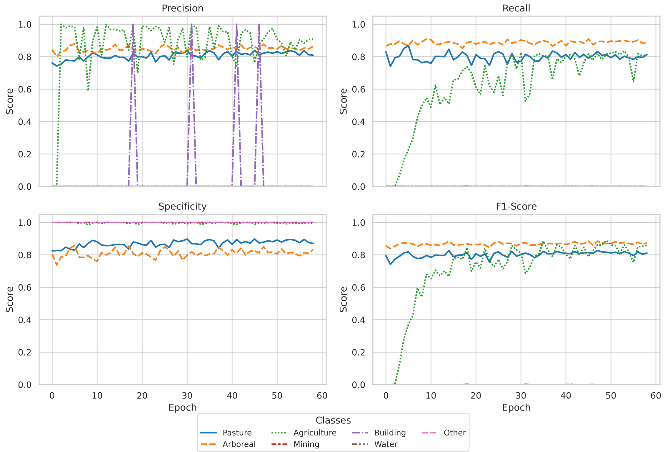
Per-Class Metrics Over Epochs
