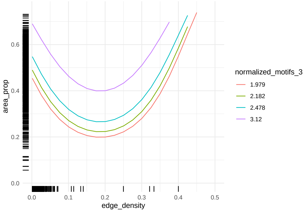
Figure 4: Estimated proportion of maximum area as a function of edge density and normalized number of motifs of size 3.
