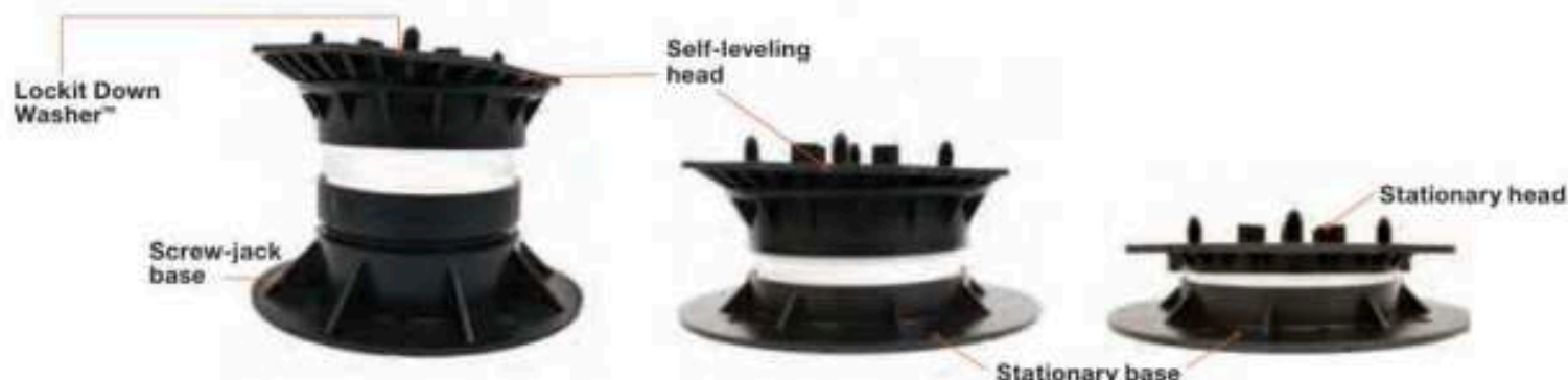
SJB-4156 SCREW-TO-ADJUST PEDESTAL 4-5/32" MIN.
