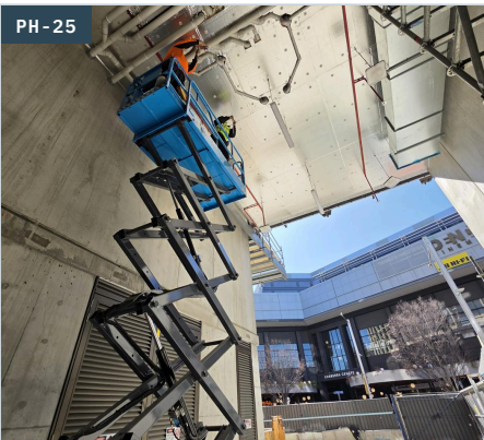
ACCESS EWP set up at Level 1 Scissor lift set up for the changeover between Level 1 and the scaffold.
