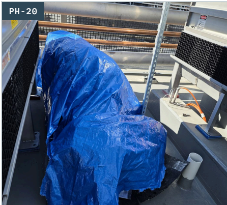
PROTECTION Second pallet covered Balance covered and weighted down against wind exposure.
