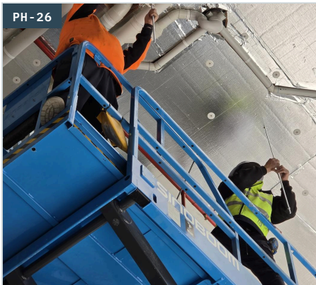
SEISMIC Parts changed from the EWP Braces and fixings changed out at the soffit from the platform.
