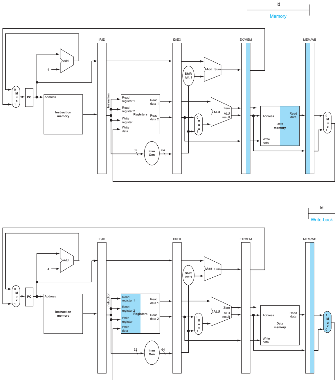
FIGURE 4.36 MEM and WB: The fourth and fifth pipe stages of a load instruction, highlighting the portions of the datapath in Figure 4.33 used in this pipe stage. Data memory is read using the address in the EX/MEM pipeline registers, and the data are placed in the MEM/WB pipeline register. Next, data are read from the MEM/WB pipeline register and written into the register file in the middle of the datapath. Note: there is a bug in this design that is repaired in Figure 4.39.
