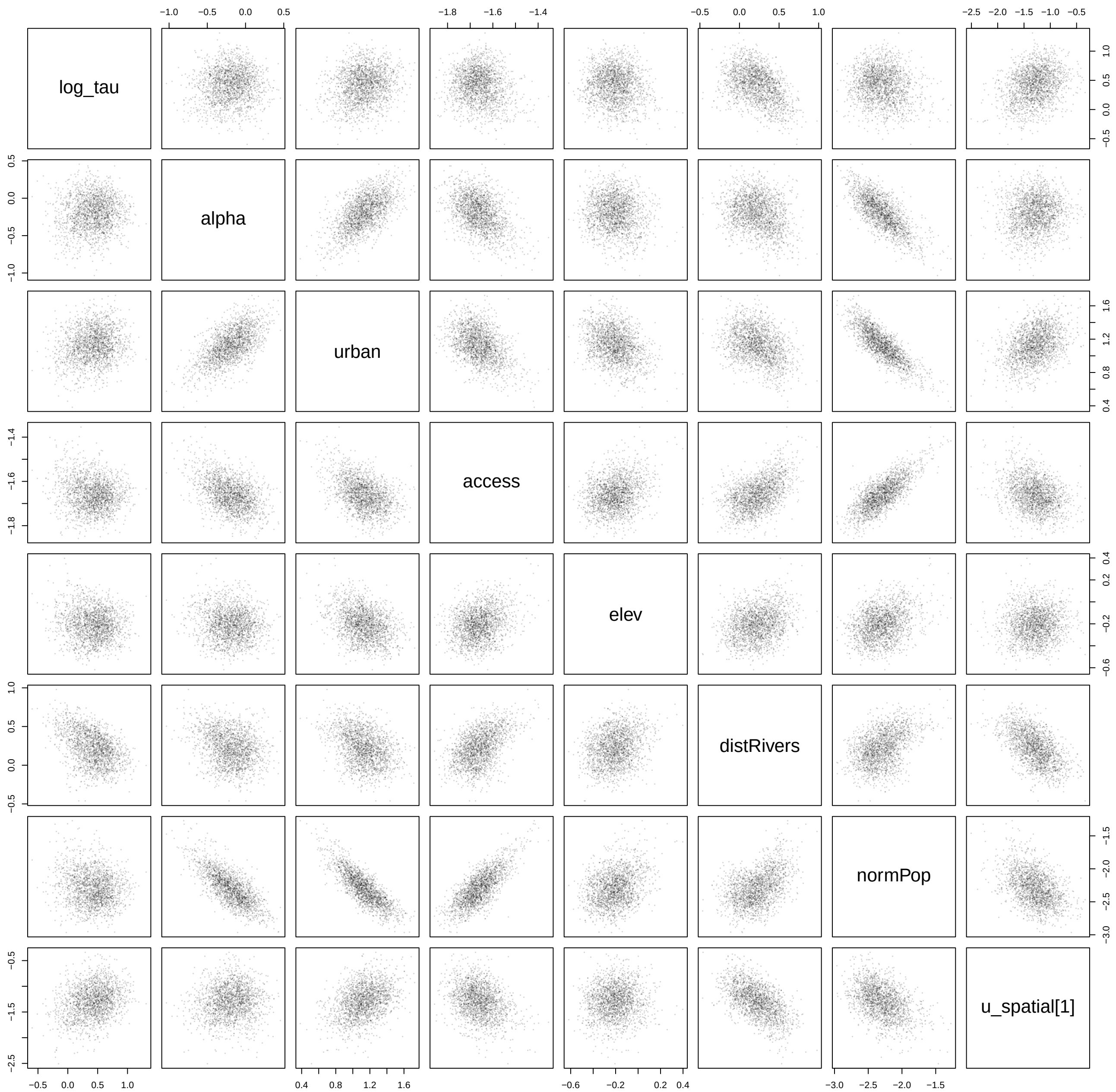
IID Model MCMC: Posterior Pair Plot
