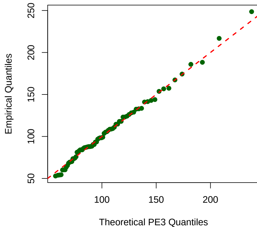
(b) PE3 Distribution (eta = 1)
