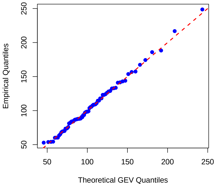
(a) GEV Distribution (eta = 1)
