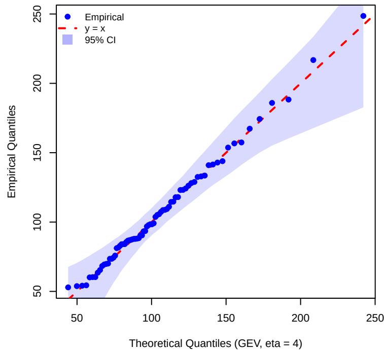
GEV Q-Q Plot (eta = 4 )
