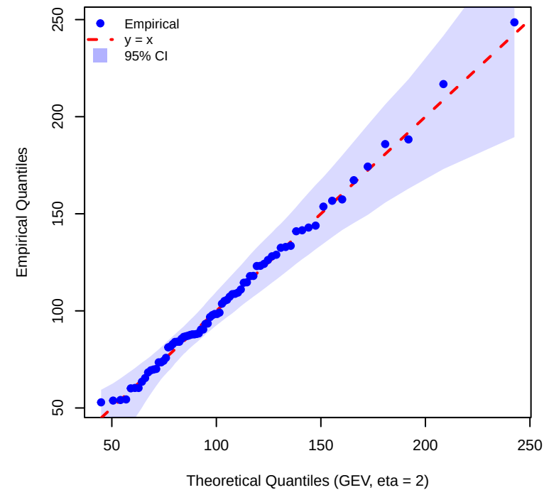
GEV Q-Q Plot (eta = 2 )
