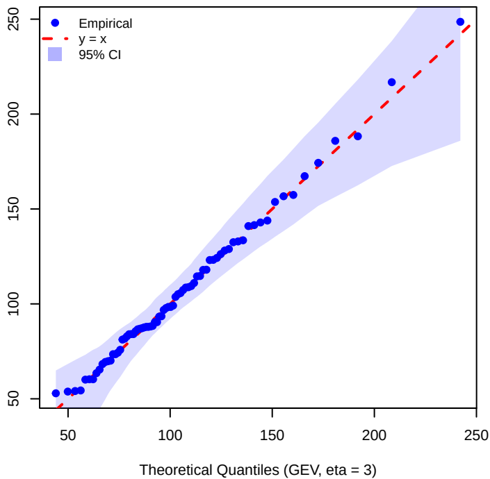
GEV Q-Q Plot (eta = 3 )
