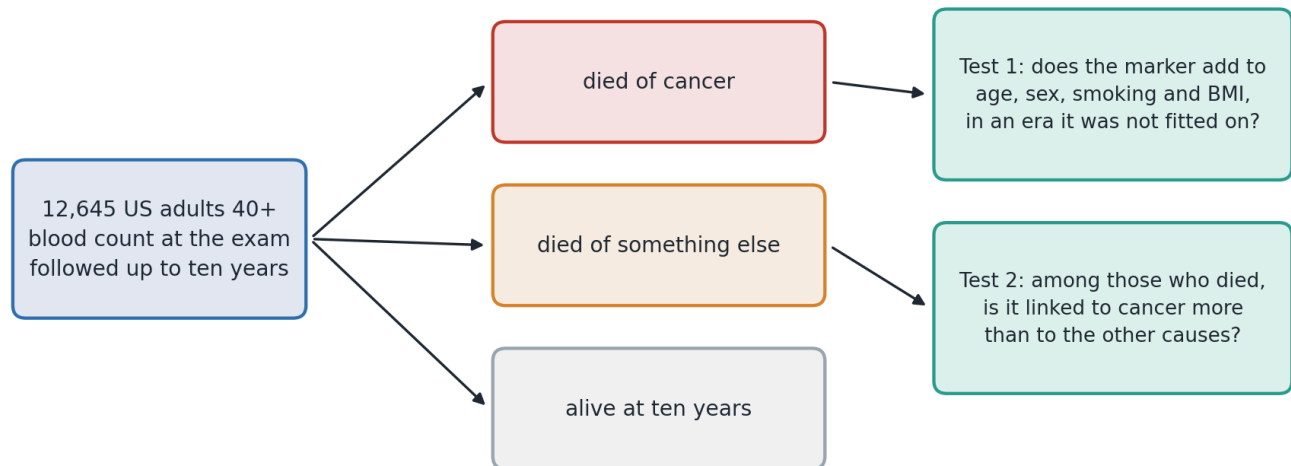
Figure 1. The design. Everyone is classed as died of cancer, died of something else, or alive at ten years. The test asks whether a marker is about cancer rather than about being unwell.
