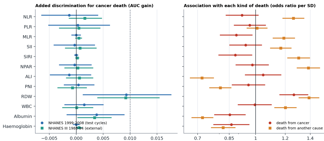
Figure 6. The main test cycles (blue) and an independent survey (teal) side by side. Left: AUC gain for cancer death. Right, from NHANES III: odds ratios per SD for death from cancer (red) and from other causes (orange). The picture is the same.
