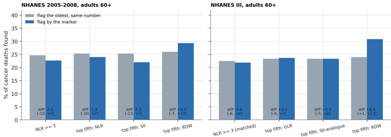
Figure 7. Share of ten-year cancer deaths found by flagging about a fifth of adults 60 and over, by the marker (blue) and by age alone (grey), with the difference and its 95% interval under each pair.
