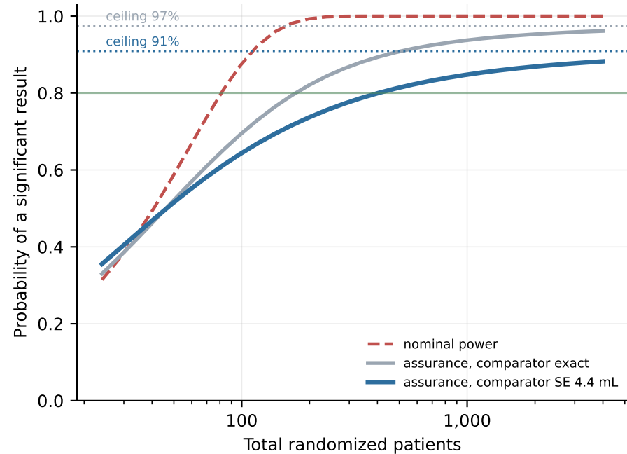
Nominal power overstates the real chance of success
