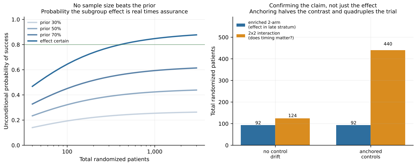
Figure 7: Left: unconditional probability of success is the prior on the subgroup effect times the assurance, so no sample size beats the prior. Right: the cost of confirming that timing matters, rather than only that the therapy works in one stratum.
