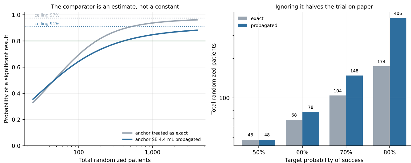
Figure 5: Treating the comparator as a constant is optimistic. Propagating its 4.4 mL standard error lowers the achievable ceiling and roughly doubles the enrollment needed for a given probability of success.
