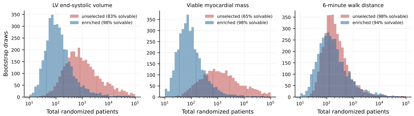
Figure 9: Bootstrap distributions of required enrollment. Intervals are wide because six to eight patients per stratum cannot pin a sample size precisely.
