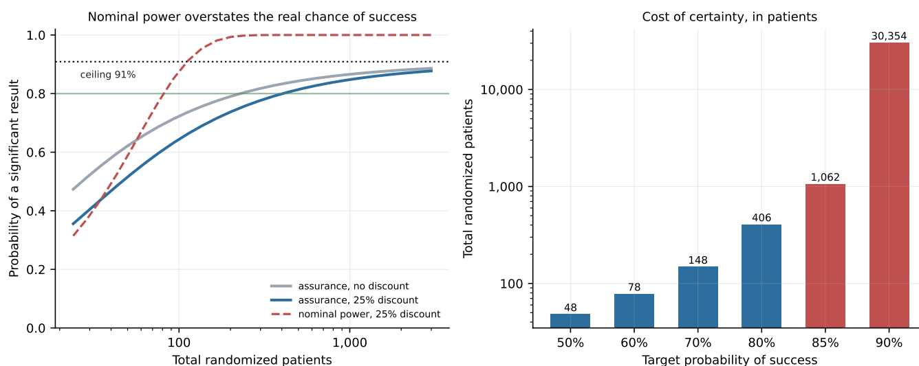
Figure 6: Nominal power against assurance, and the enrollment required for a target probability of success.
