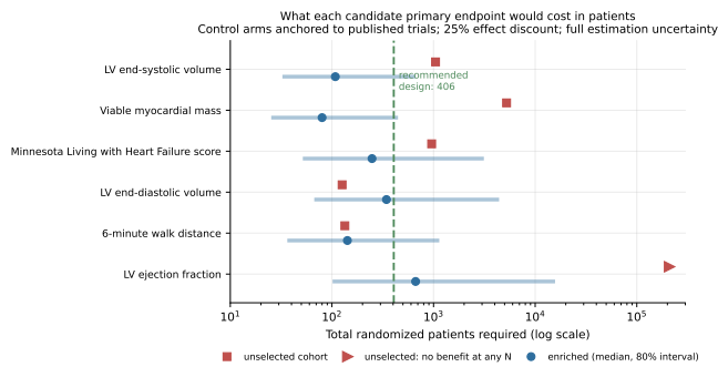
Figure 10: Required enrollment per candidate primary endpoint, with the recommended design marked.
