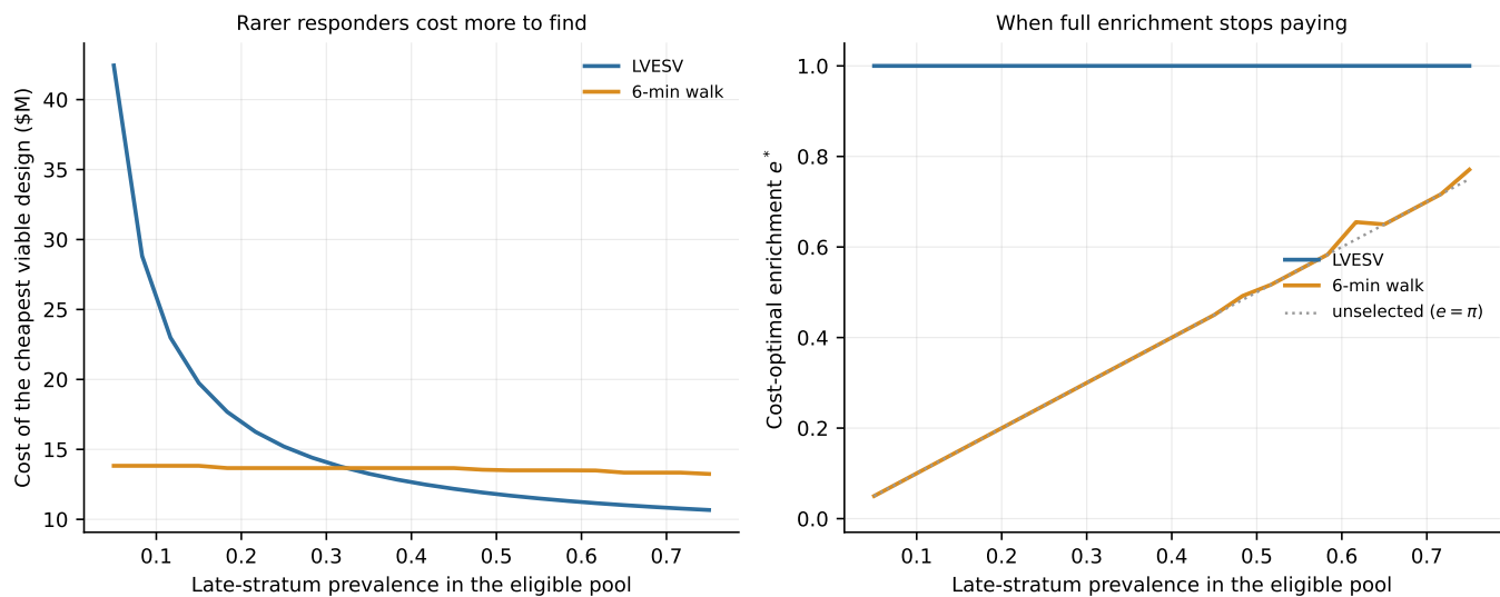
Figure 11: Cost of the cheapest viable design as responders become scarcer, and the enrichment level at which full enrichment stops paying.
