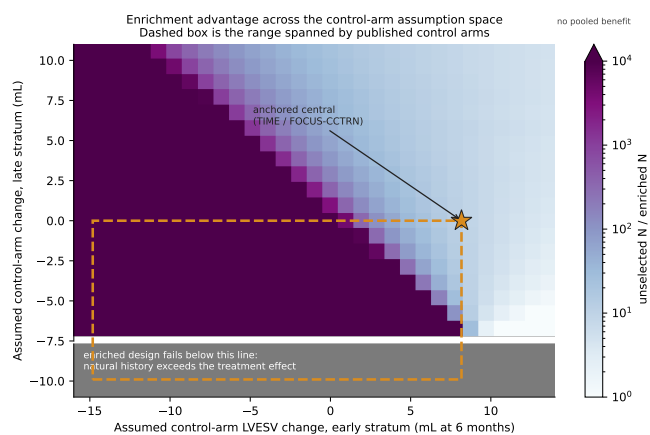
Figure 8: Enrichment advantage across the comparator assumption space. Below the white line the enriched design fails outright, because assumed natural history exceeds the treatment effect.
