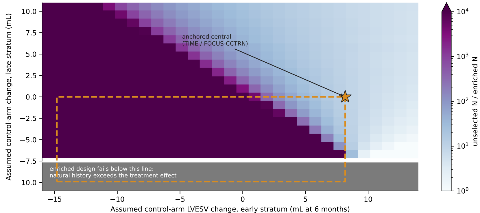
Enrichment advantage across the control-arm assumption space Dashed box is the range spanned by published control arms
