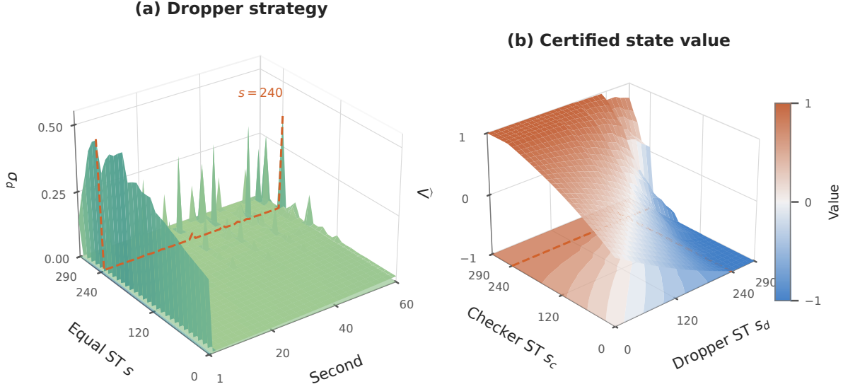
Figure 5: Two zero-TTD slices, sampled in 10-second ST steps; dashed lines mark the survival boundary at ST 240. (a) The Dropper's equilibrium mix along (s, 0, s, 0) . Every sampled strategy has full support, with an atom on second 1 at every ST value; the boundary at s = 240 adds a second atom on second 60, and the mix flattens near overflow. (b) Certified values \hat{V}(s_c, 0, s_d, 0) . At equal ST values of 290 the Dropper's value is 0.753; unequal high ST values create the opposing cliffs.
