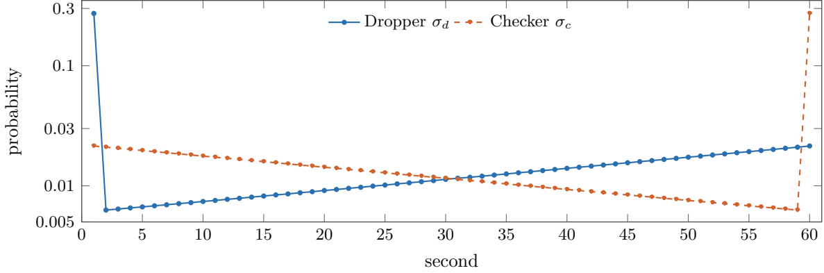
Figure 4: The certified equilibrium at the initial state (0, 0, 0, 0) ; the displayed pair's saddle gap against the full matrix is 3.2 \times 10^{-15} . Both strategies are full-support. The Dropper concentrates 27.3% on dropping immediately and shades the remainder toward later seconds; the Checker mirrors it. The logarithmic axis keeps the atom and the remaining support visible together.
