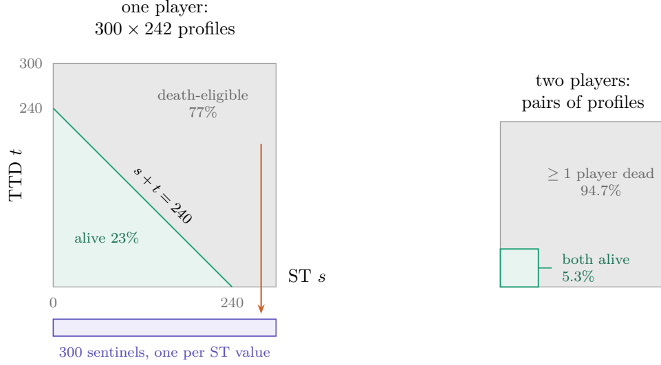
Figure 3: The geometry of the quotient. Left: the alive triangle contains 16,711 of 72,600 profiles; at each ST value, all dead TTD values map to one of 300 sentinels, leaving 17,011 classes. Right: applying the map to both players reduces the 5.27 \times 10^9 domain states to 289,374,121, a factor of 18.2. Left-panel areas are schematic: the unreachable TTD band 1..59 (Lemma 4.4) is drawn as part of the continuum; the percentages are exact counts.
