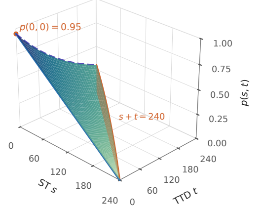
Figure 1: Revival becomes less likely as either time total grows. Beyond s + t = 240 , the player cannot survive; at s = 240 , revival also has probability zero.
