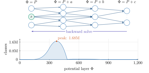
Figure 4: Play moves to higher layers; we solve in reverse. The widest layer contains 1,678,715 classes.
