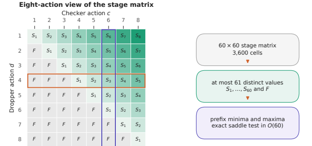
Figure 2: Each diagonal has one success payoff S_\ell ; each failed check has payoff F . We need at most 61 values for the 3,600 action pairs.
