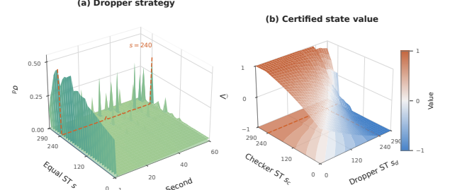
Figure 5: With both TTDs zero: the Dropper's strategy \sigma_d = a at equal ST (left), and the game value as each player's ST changes (right).
