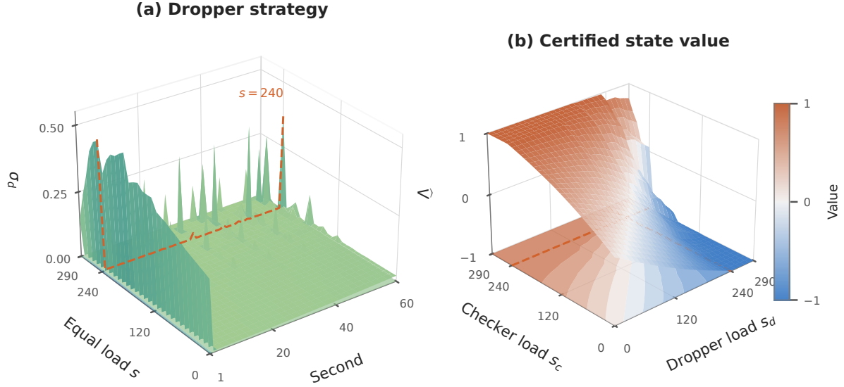
Figure 5: Two zero-TTD slices, sampled in 10-load steps; dashed lines mark the survival boundary at load 240. (a) The Dropper’s equilibrium mix along (s, 0, s, 0) . Every sampled strategy has full support, with an atom on second 1 at every load; the boundary at s = 240 adds a second atom on second 60, and the mix flattens near overflow. (b) Certified values \hat{V}(s_c, 0, s_d, 0) . At equal loads of 290 the Dropper’s value is 0.753; unequal high loads create the opposing cliffs.
