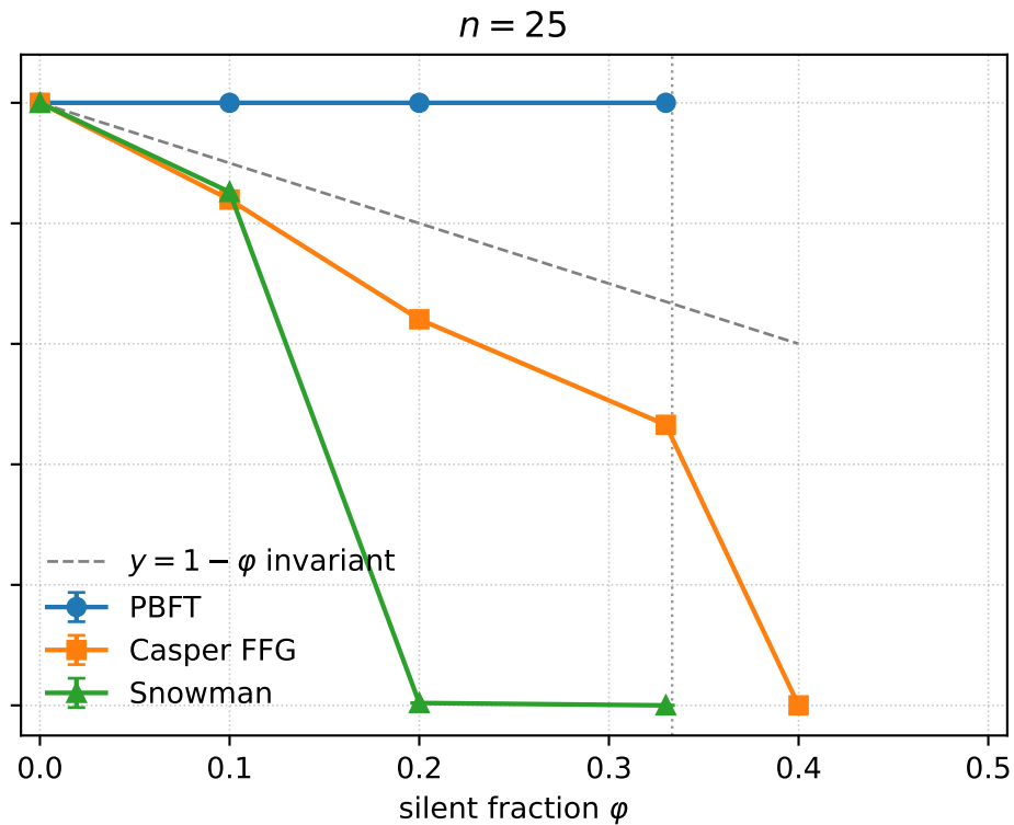
Throughput degradation under silent non-participation (mean \pm 95% CI)
