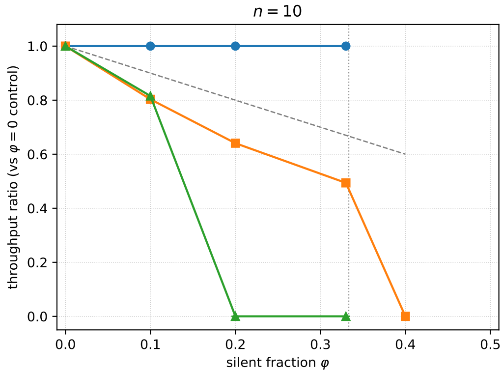
Throughput degradation under silent non-participation (mean \pm 95% CI)
