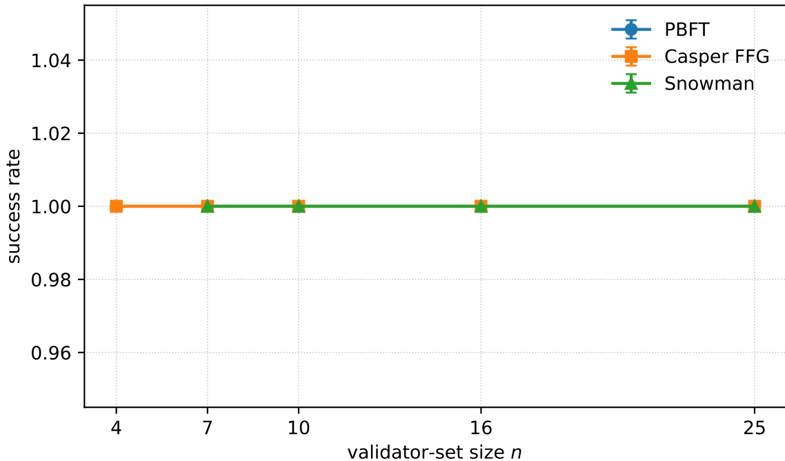
Consensus success rate vs. validator count (mean \pm 95% CI)
