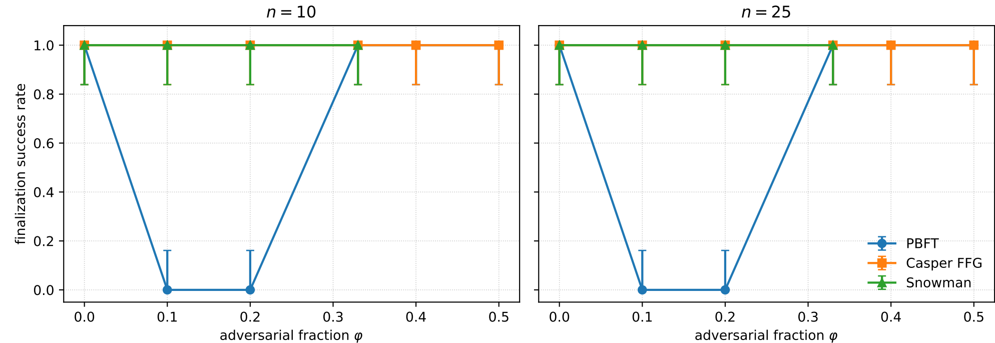
Liveness vs adversarial fraction — equivocating nodes (mean \pm 95% Wilson) (PBFT recovers via an UNSAFE fork above 1/3)
