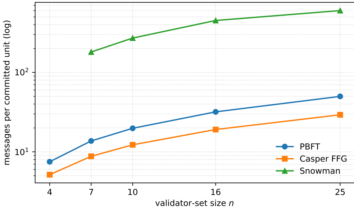
Message overhead vs. validator count
