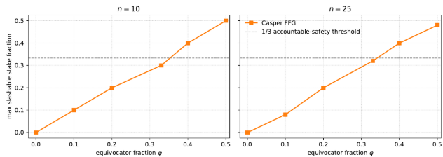
Casper FFG maximum slashable stake under equivocation
