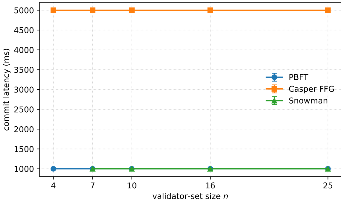
Commit latency vs. validator count (mean \pm 95% CI)
