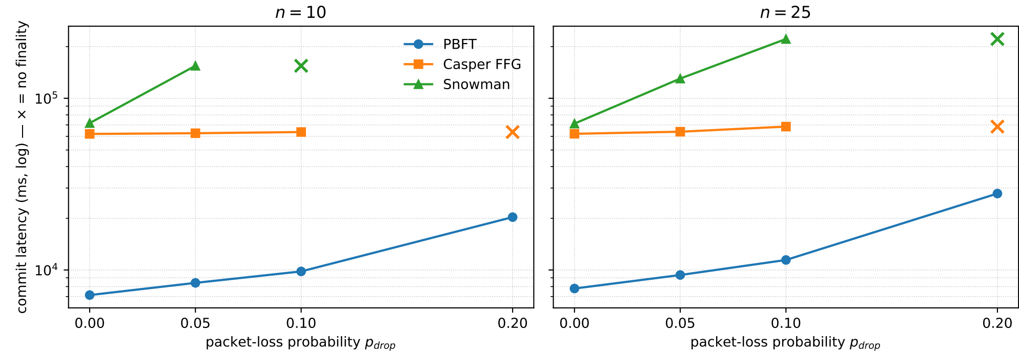
Commit-latency growth under packet loss (solid = finalizing, \times = liveness lost)
