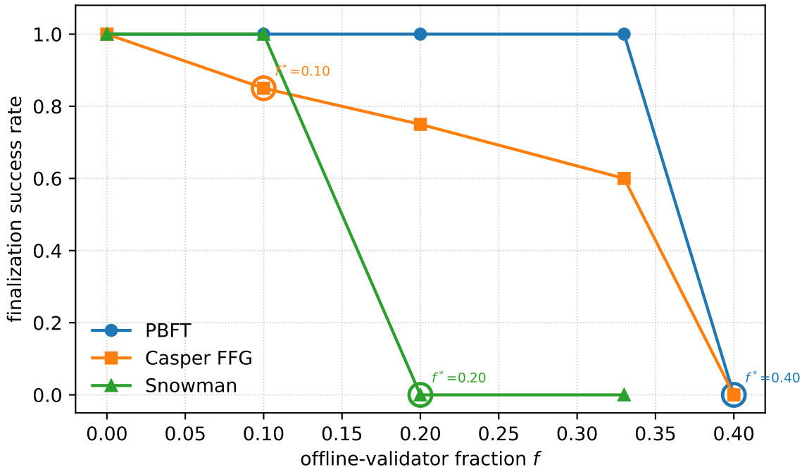
Finalization success vs offline fraction ( n = 10 , mean over 20 seeds)
